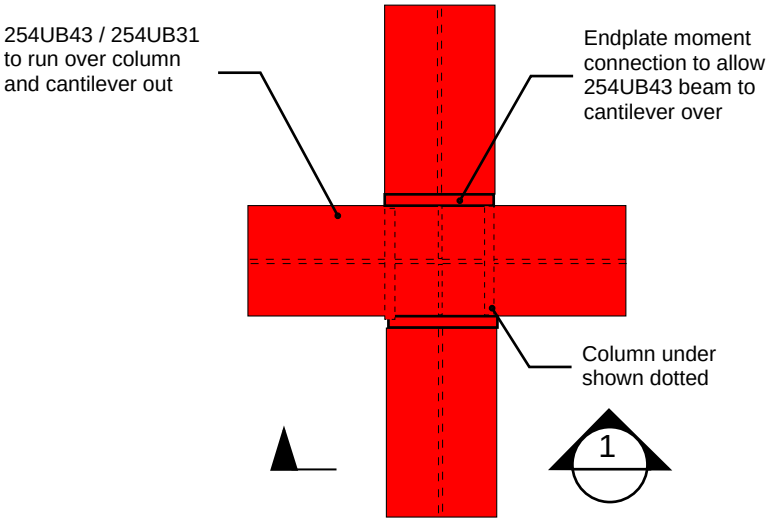
Detail A - 0100 Typical connection at column head
