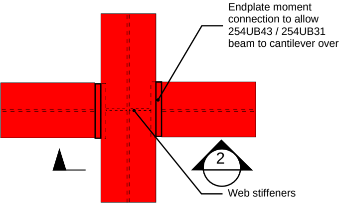
Detail B - 0100 Typical Moment Connection
