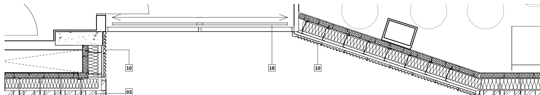
DETAIL PLAN AA
