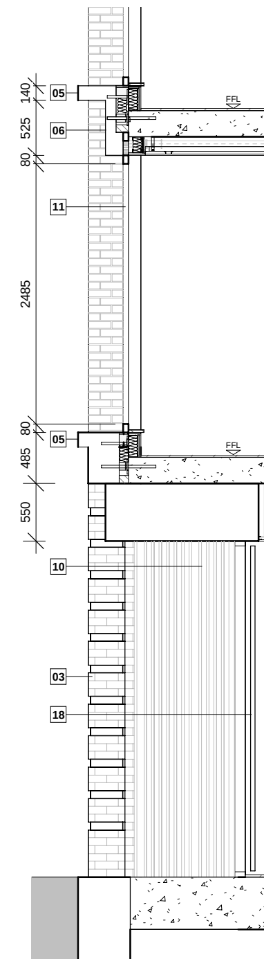
DETAIL SECTION AA
