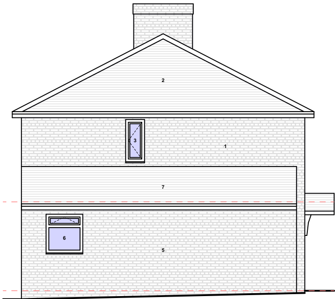
PROPOSED GA SIDE ELEVATION 1 @1:100
