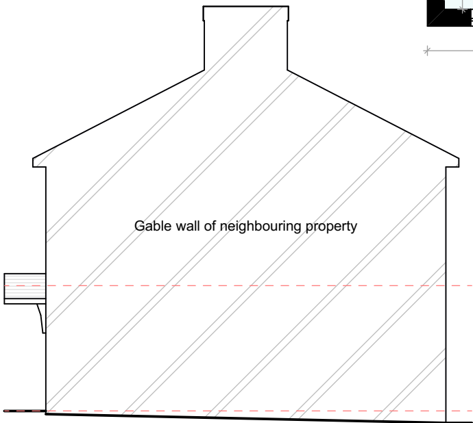
PROPOSED GA SIDE ELEVATION 2 @1:100
