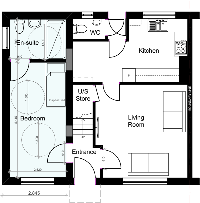
PROPOSED GA GROUND FLOOR PLAN @1:100
