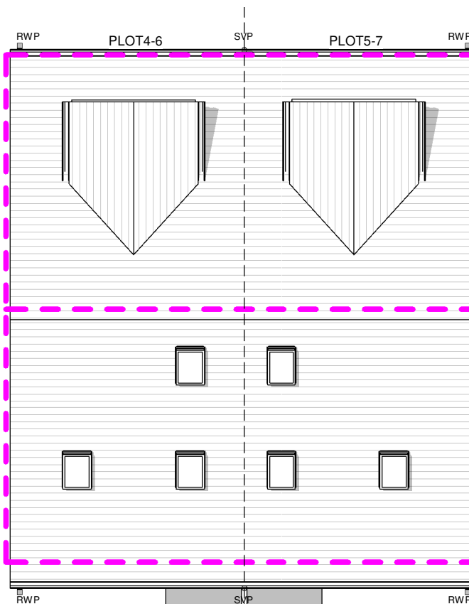
4 As-built Roof Plan 1 : 100
