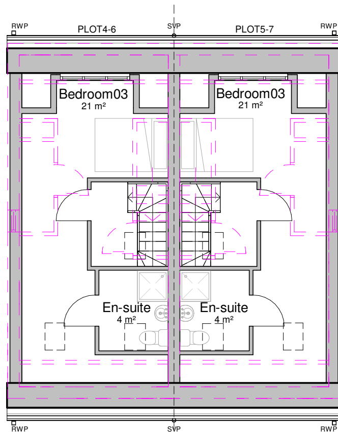
3 As-built Loft Plan 1 : 100
