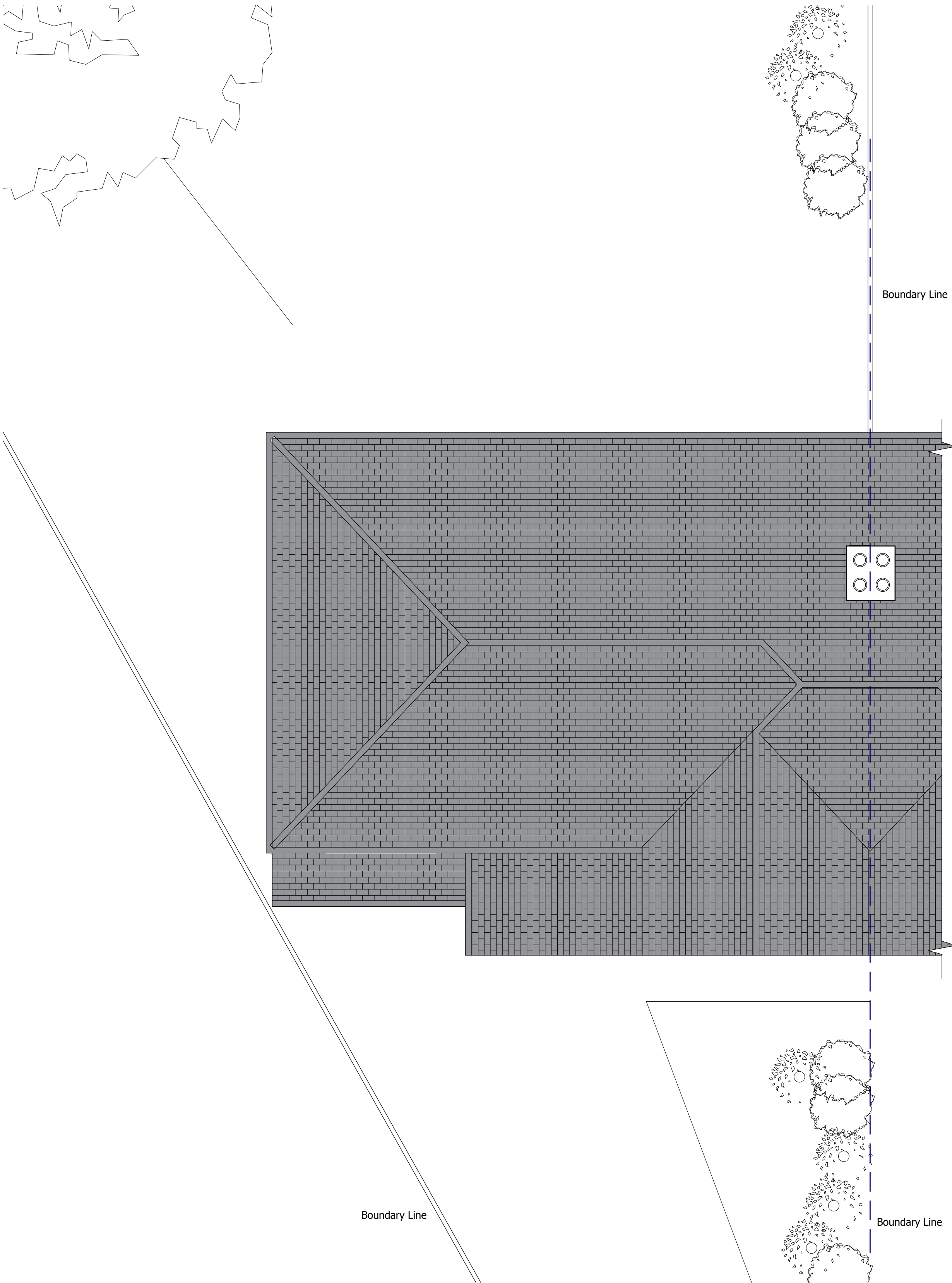
Roof Plan
