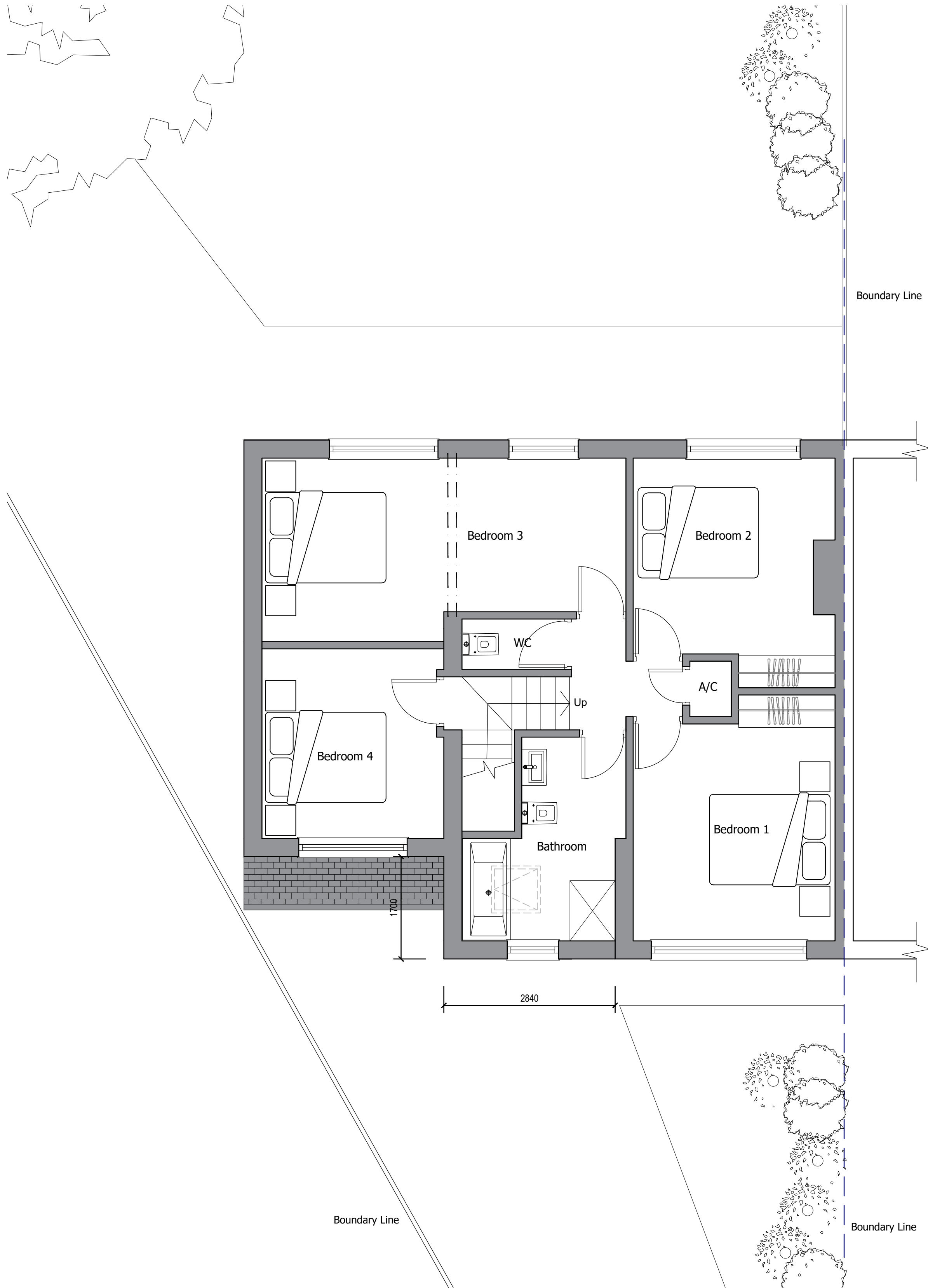
First Floor
