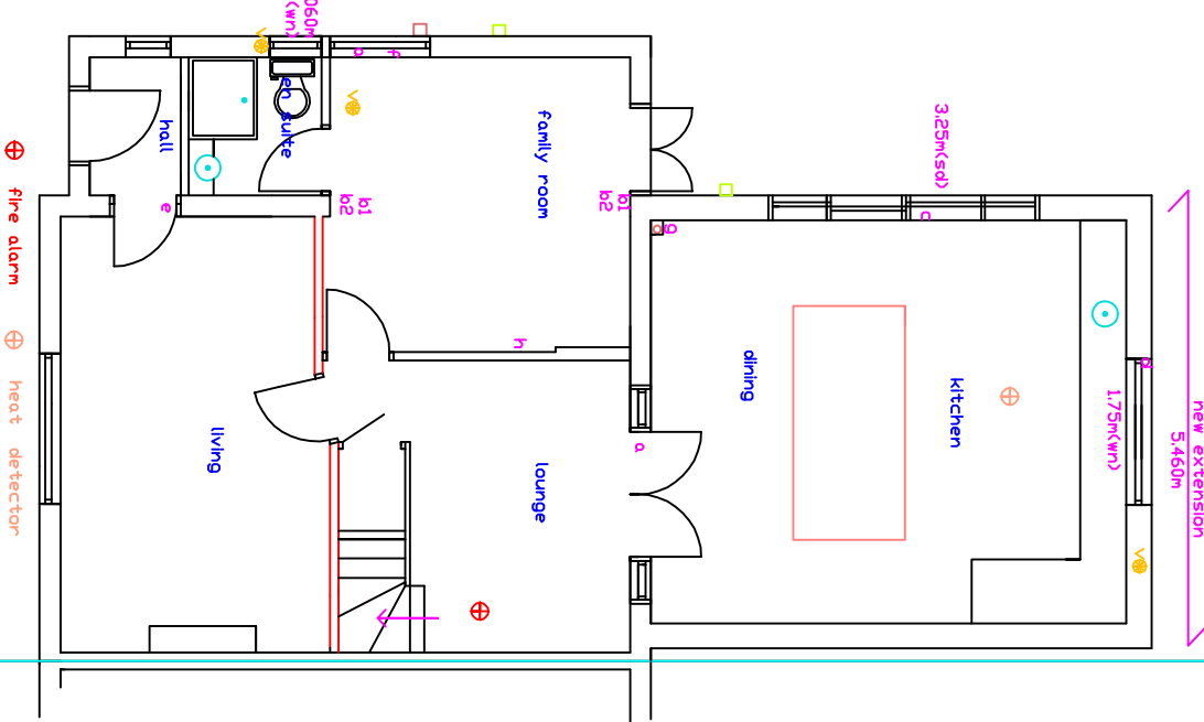
PROPOSED GROUND FLOOR 1:100
