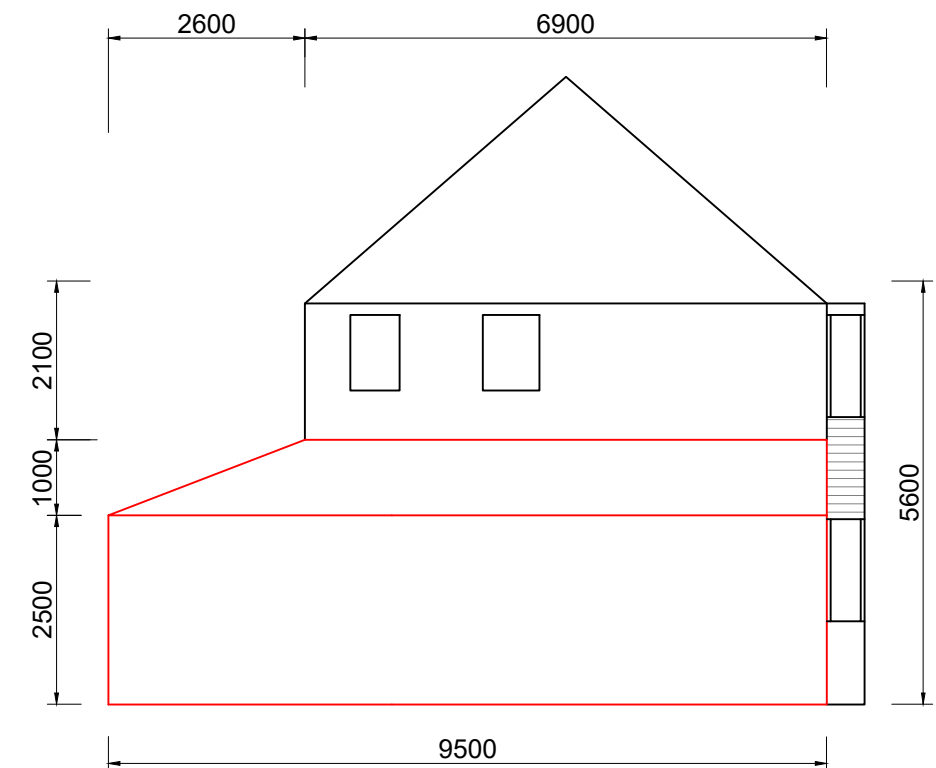
South Elevation as Proposed
