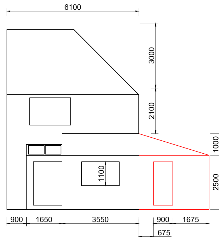
Rear Elevation as Proposed
