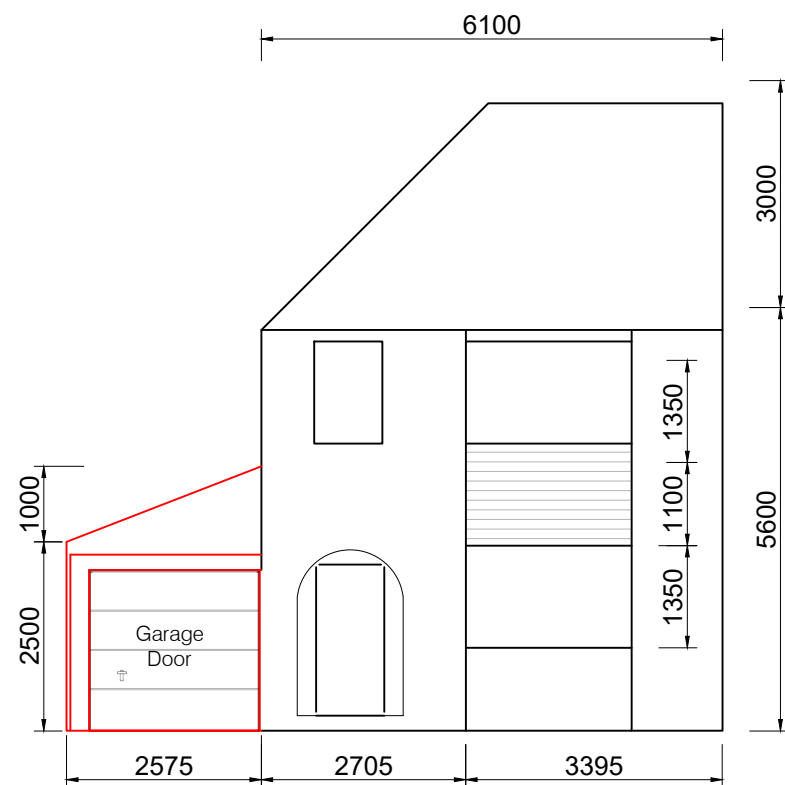
Front Elevation as Proposed
