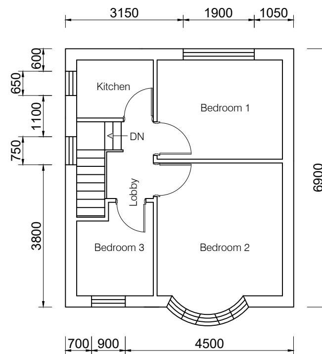
First Floor Plan as Existing (No Changes)
