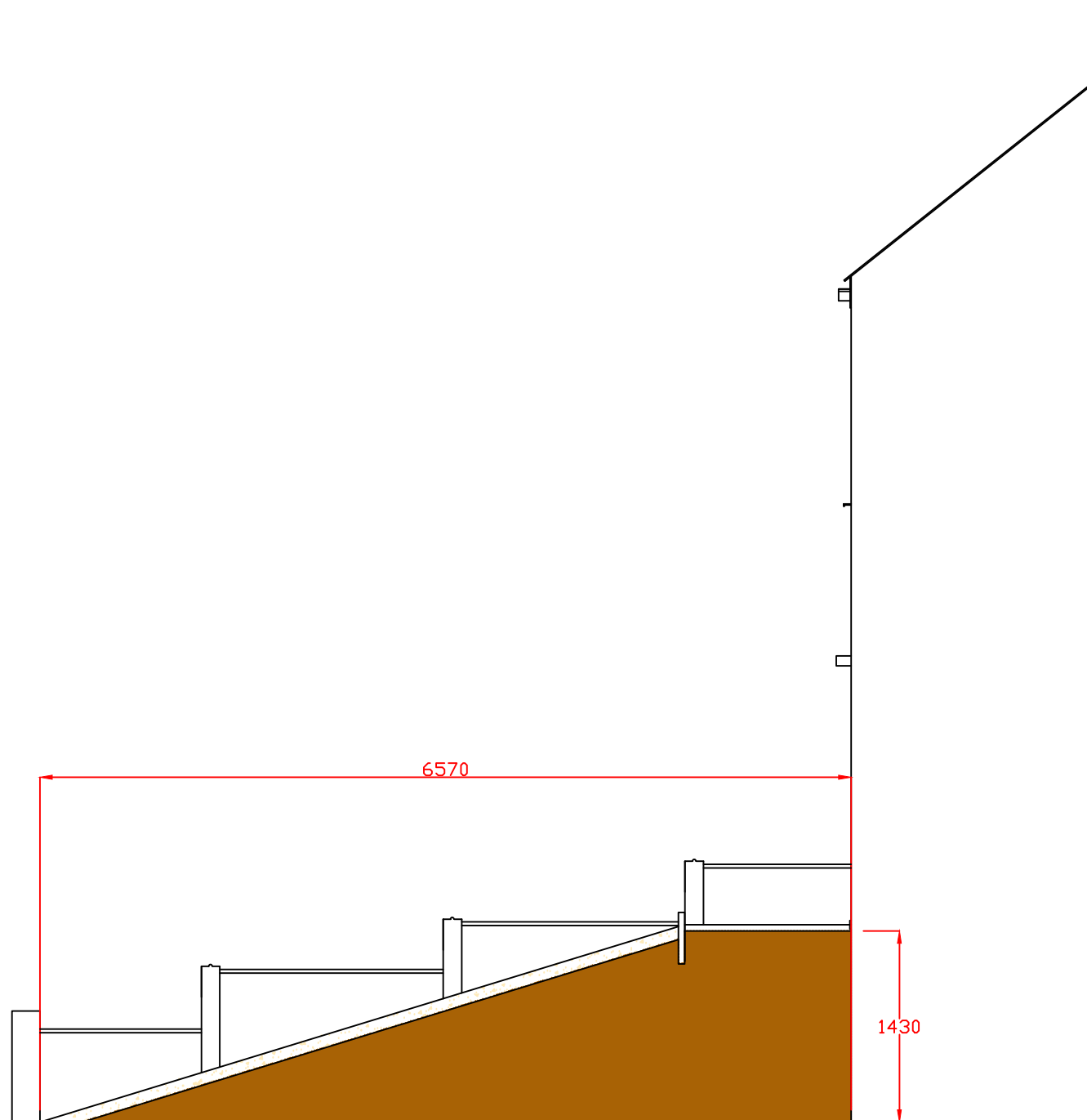
EXISTING SIDE ELEVATION VIEWED FROM NO 7
