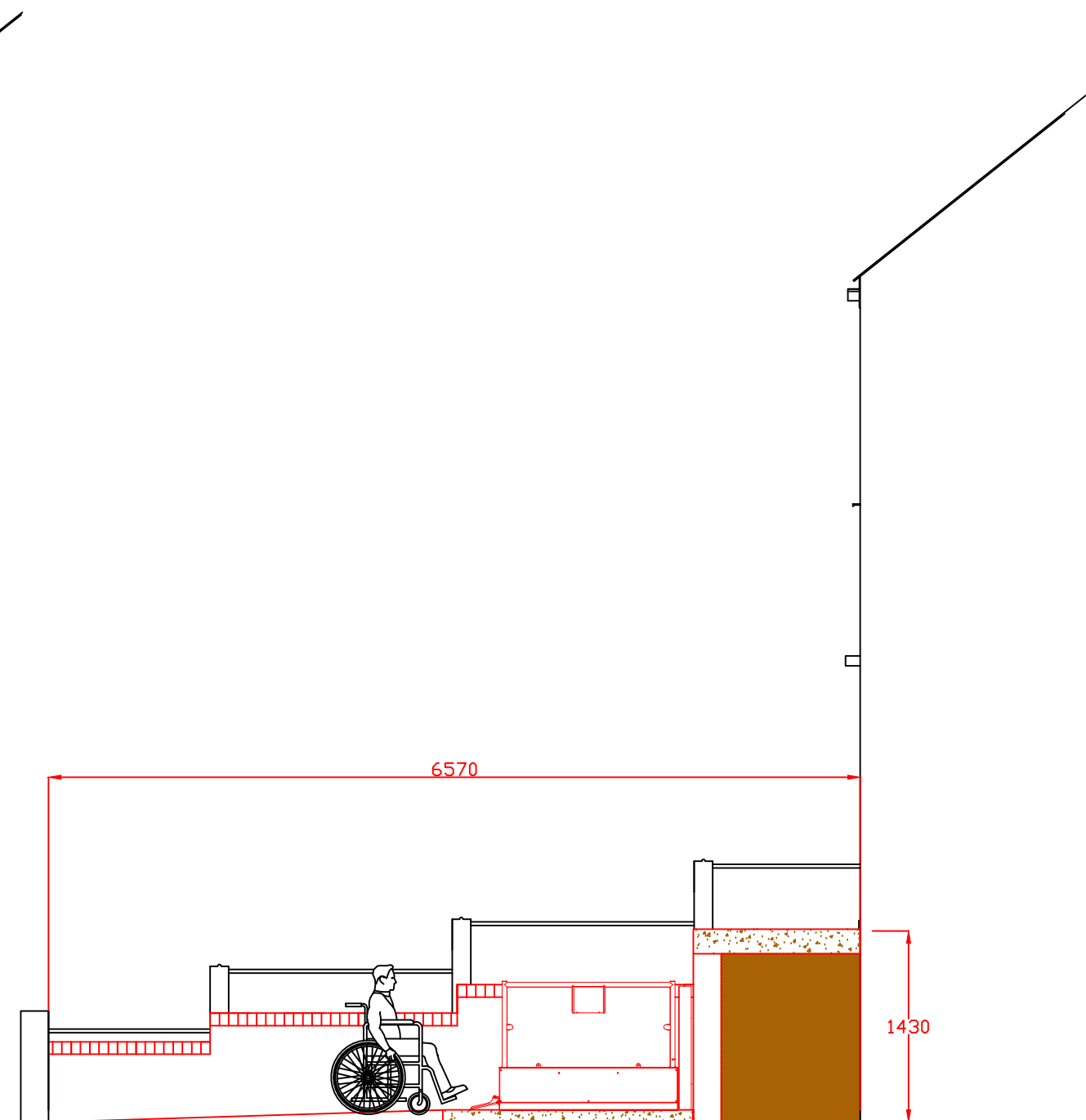
PROPOSED SIDE ELEVATION VIEWED FROM NO 7
