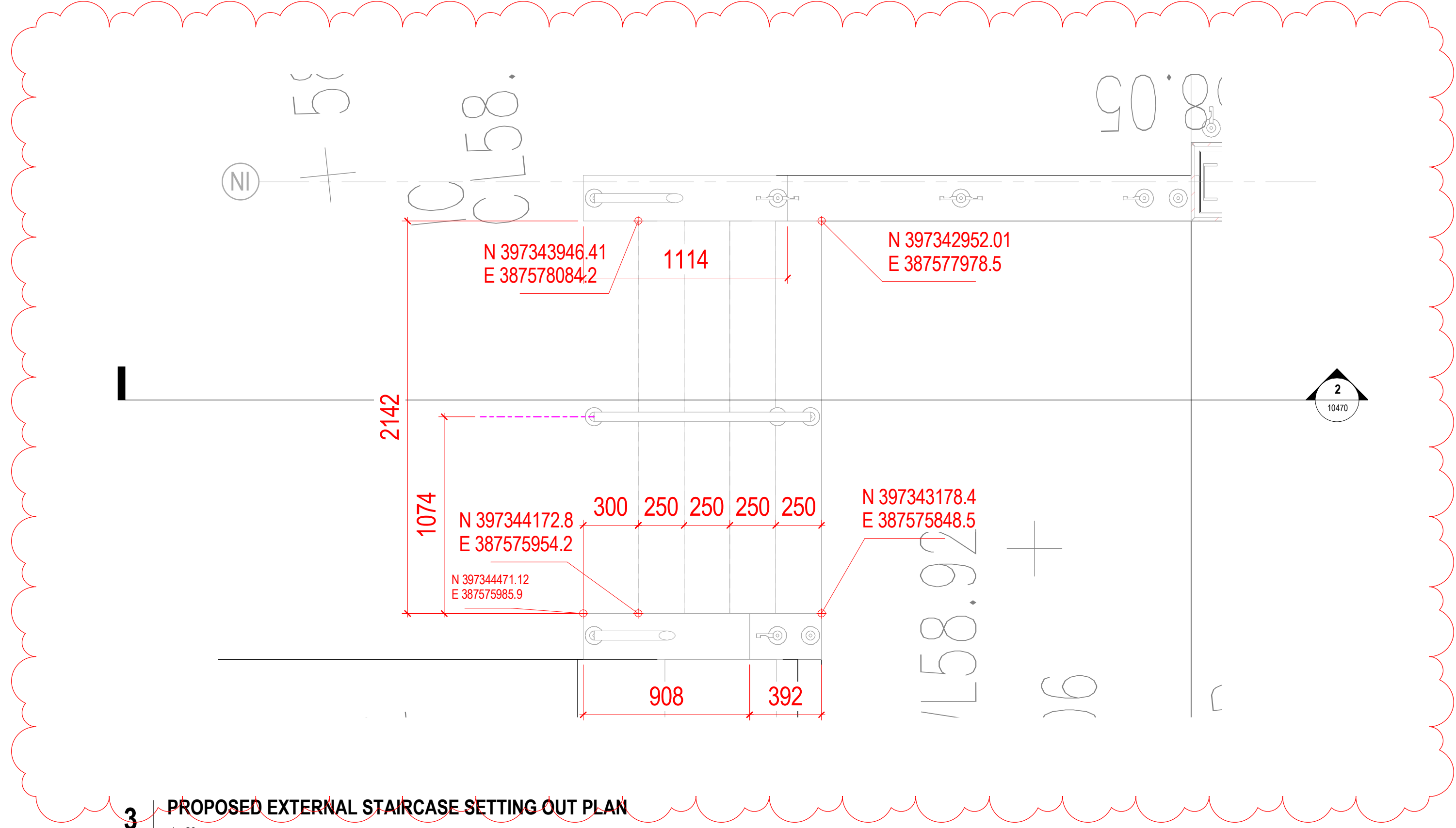
3 PROPOSED EXTERNAL STAIRCASE SETTING OUT PLAN 1:20
