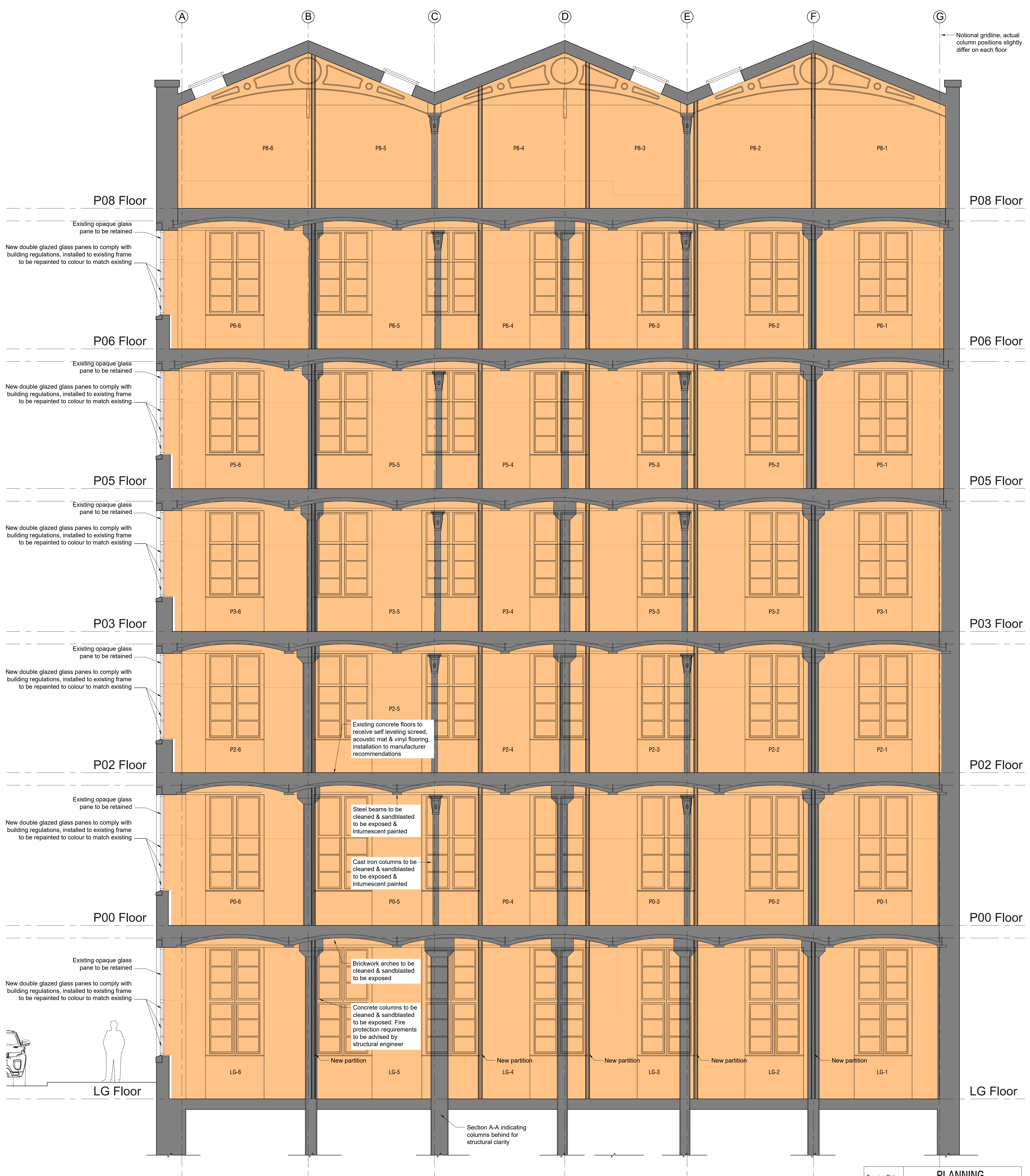
Proposed Section A-A Scale 1:50
