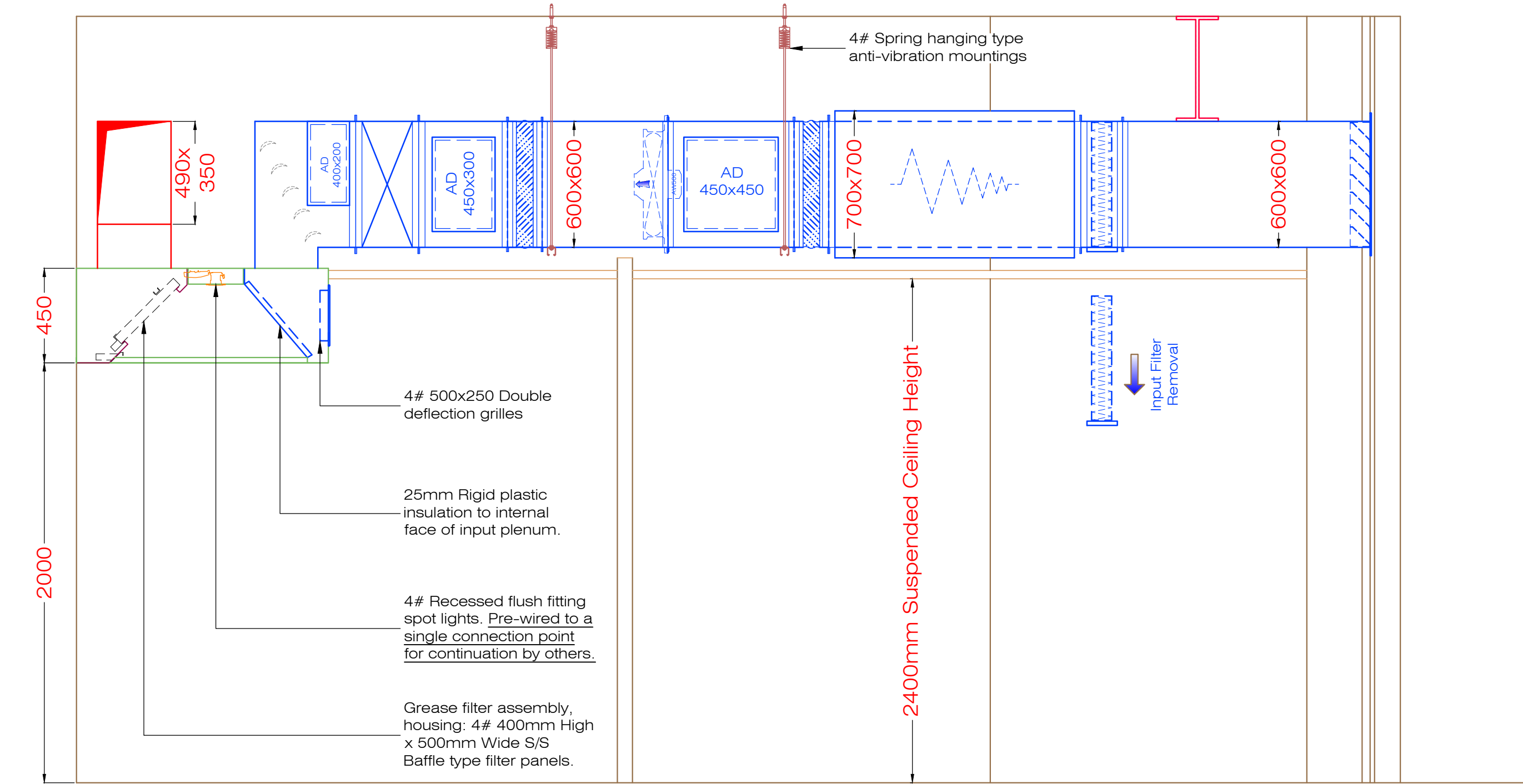
Section B-B
