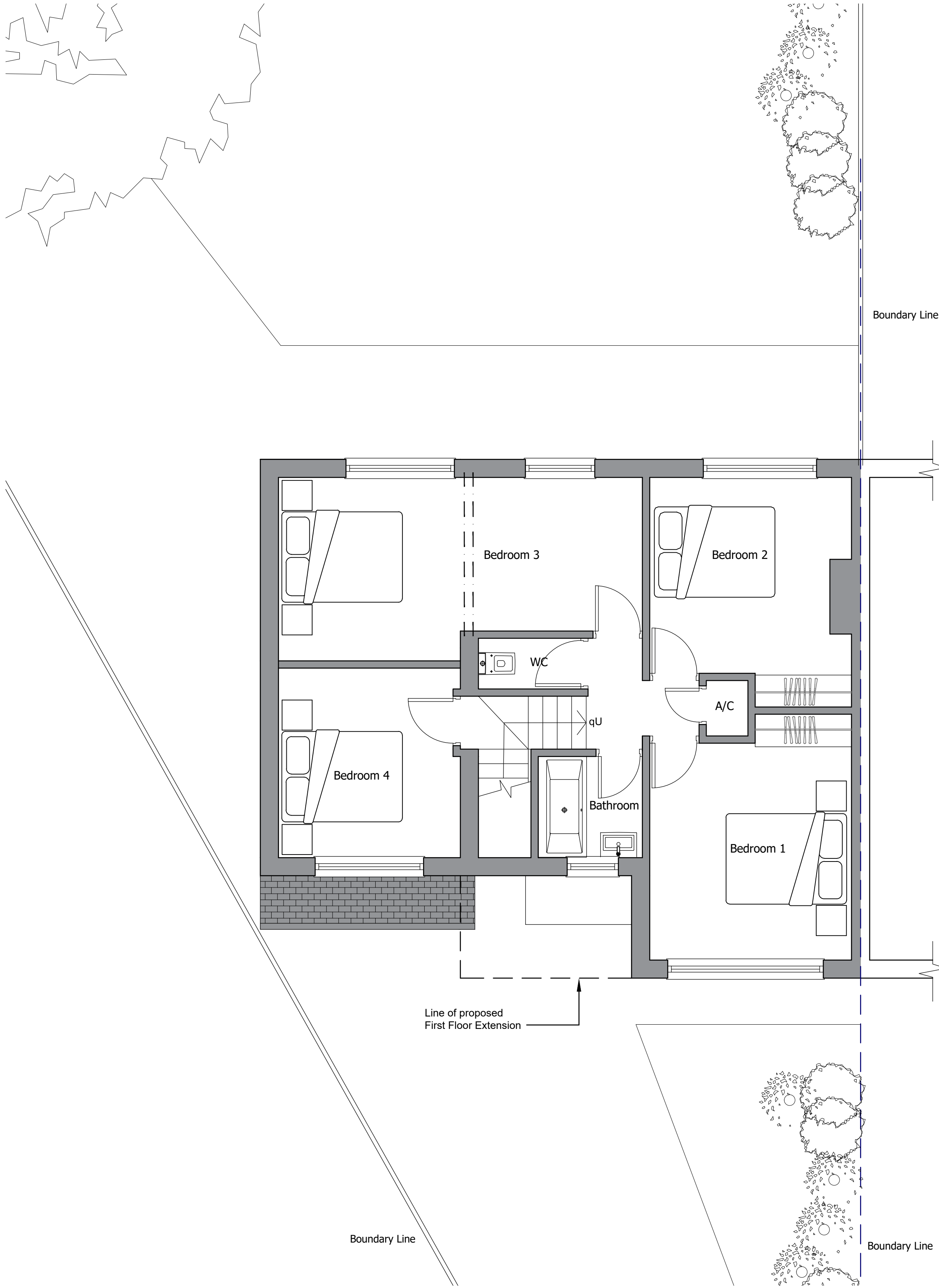
First Floor
