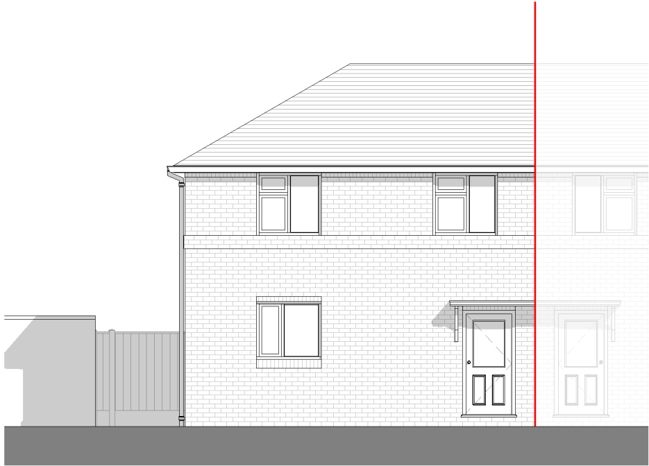
Front Elevation 1 : 100
