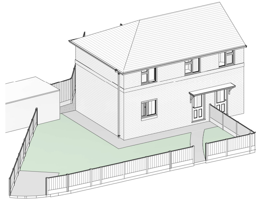
Existing Front View
