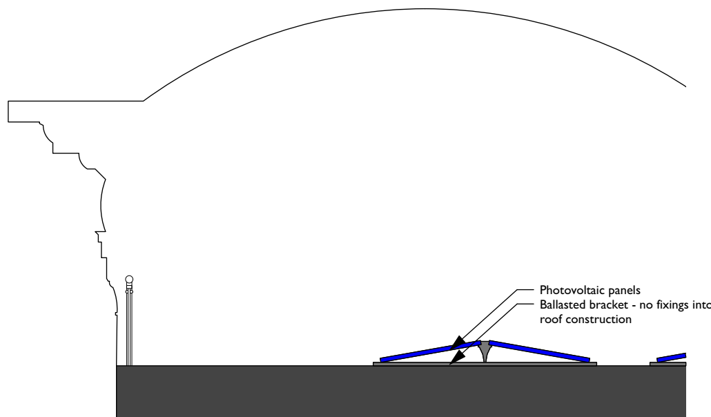
4 Localised Section Scale: 1:50
