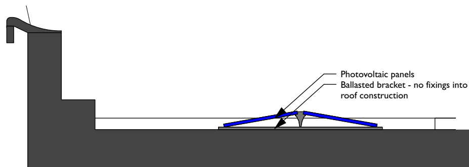
2 Localised Section Scale: 1:50
