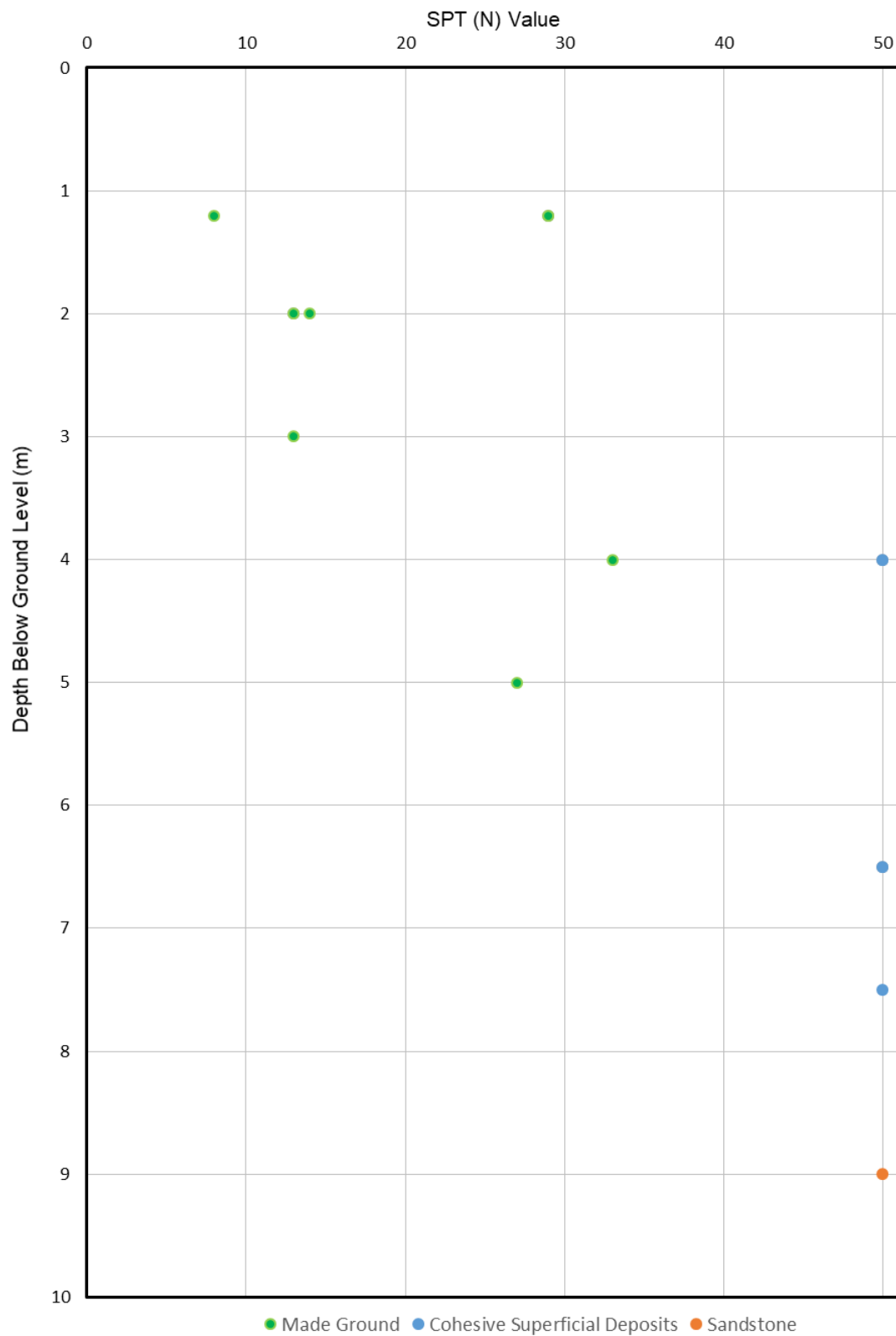
Figure 5: SPT v Depth Plot
