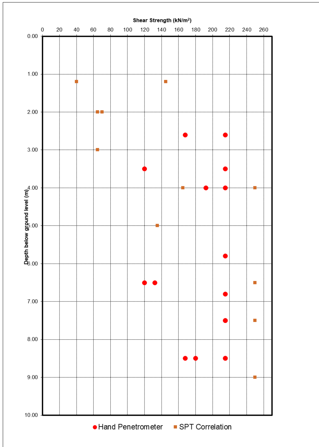
Figure 6 Strength v Depth Plot (Cohesive Superficial Deposits)
