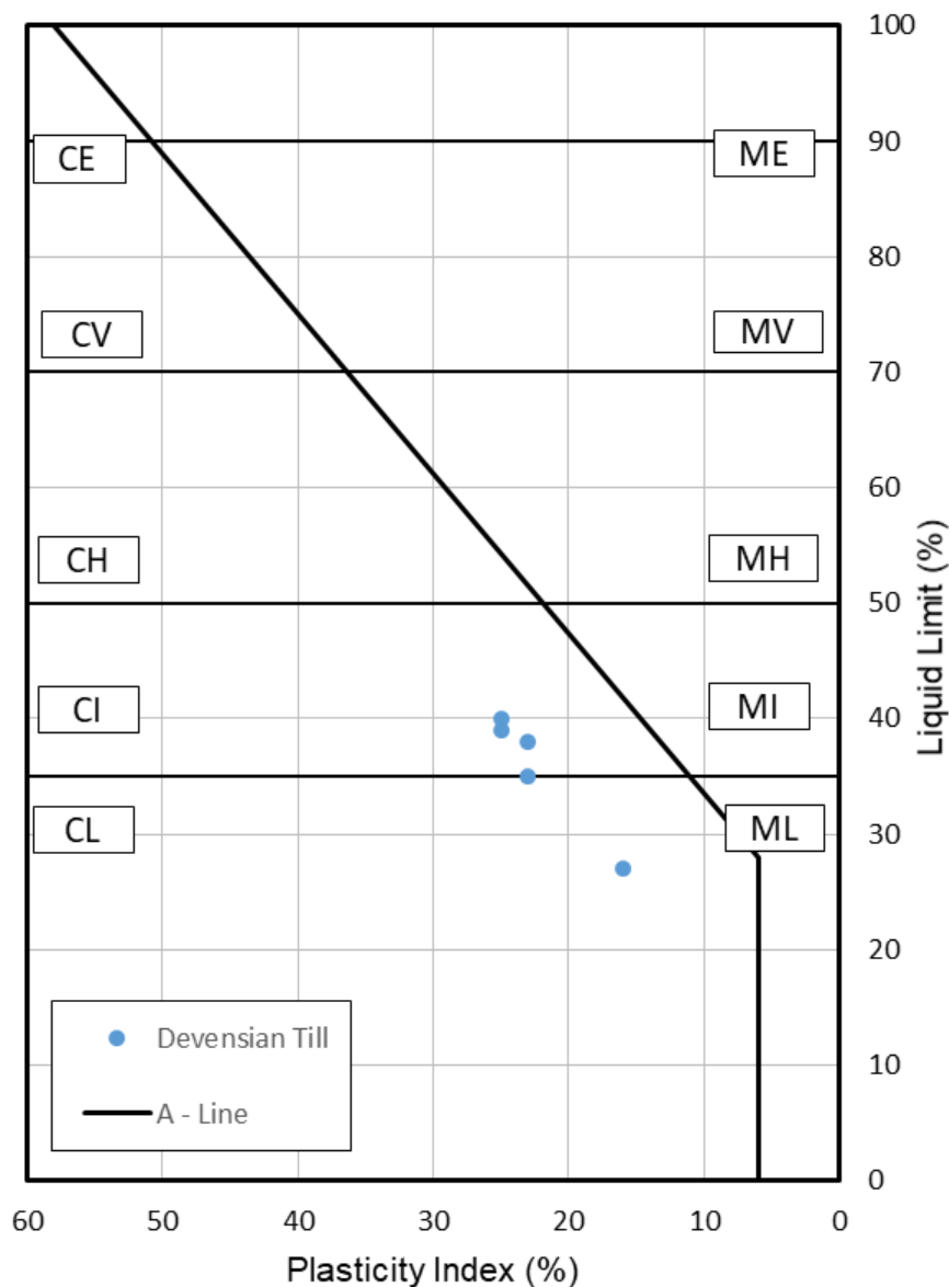
Figure 7: Plasticity Chart
