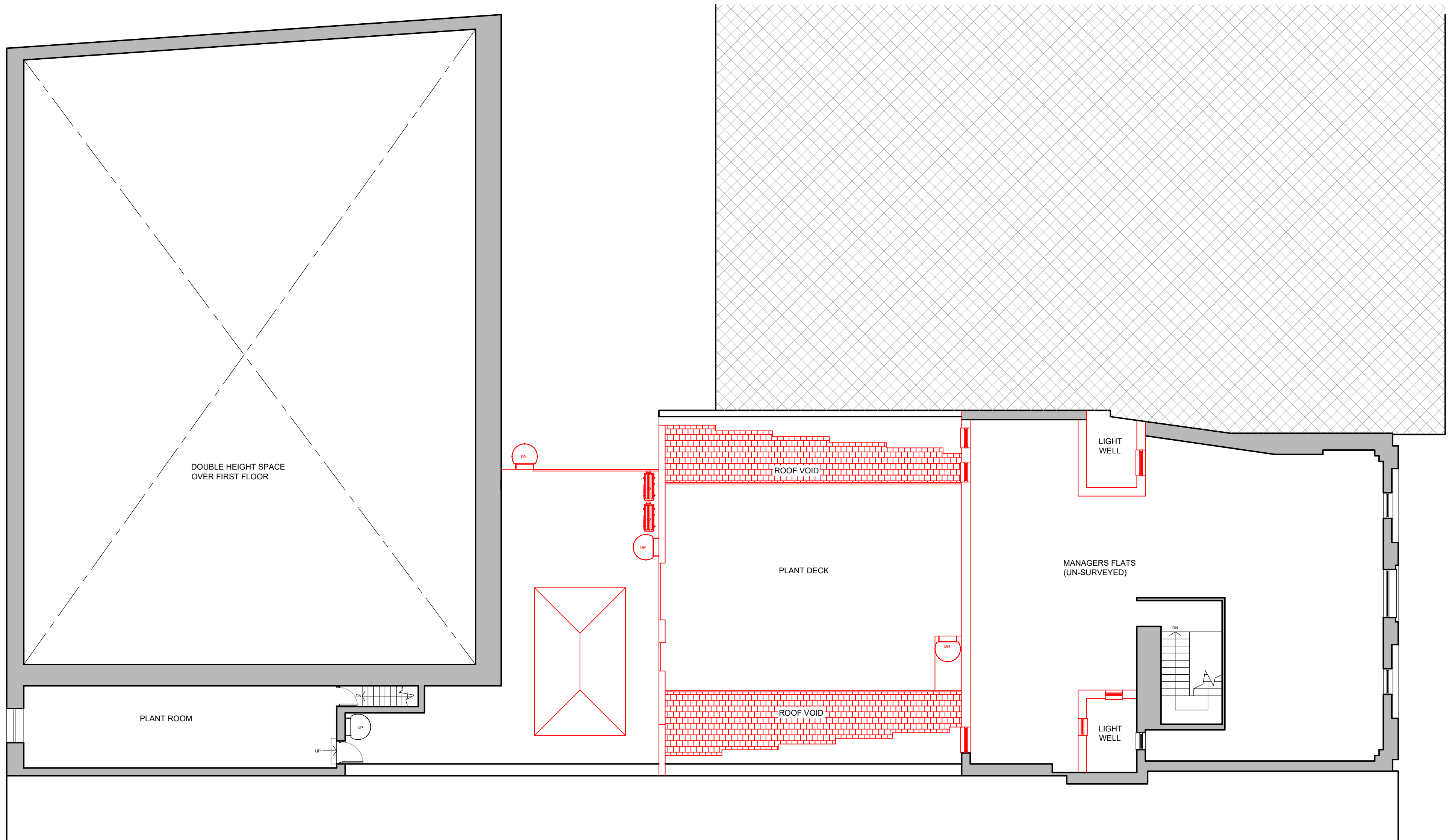
SECOND FLOOR DEMOLITION PLAN SCALE 1:100
