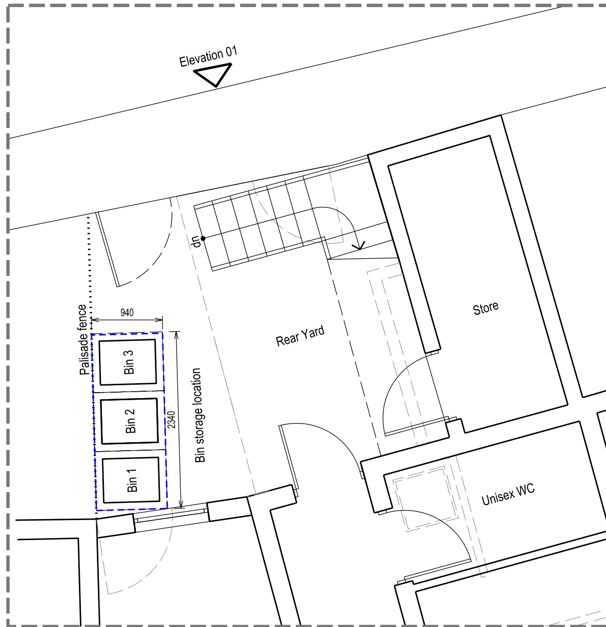
Proposed Bins Storage Plan @1/50
