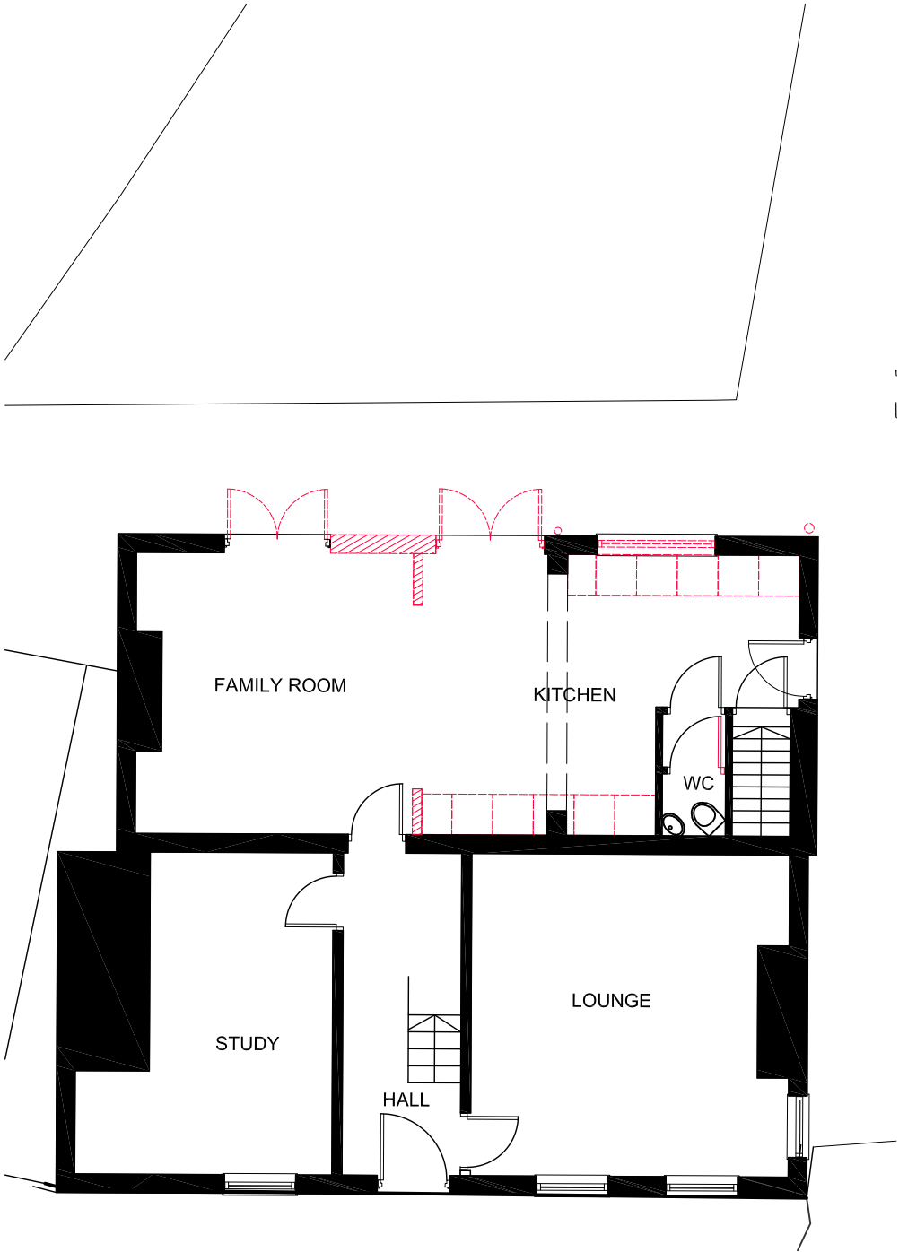
Ground Floor Plan Removals
