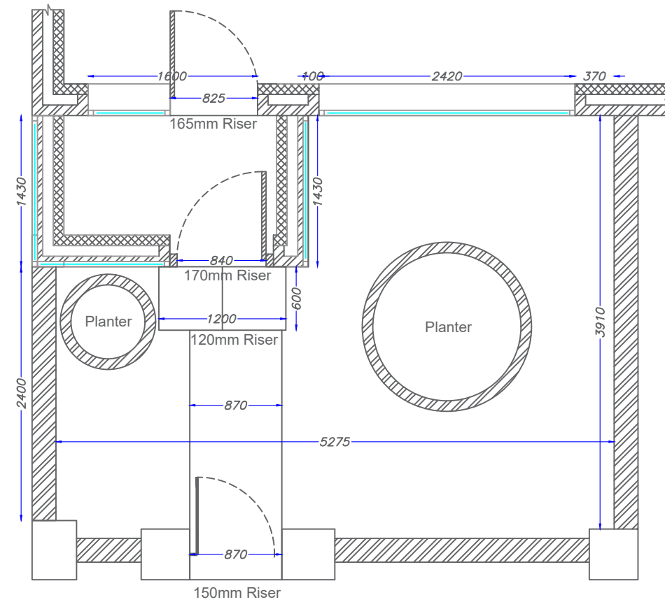
Existing Layout
