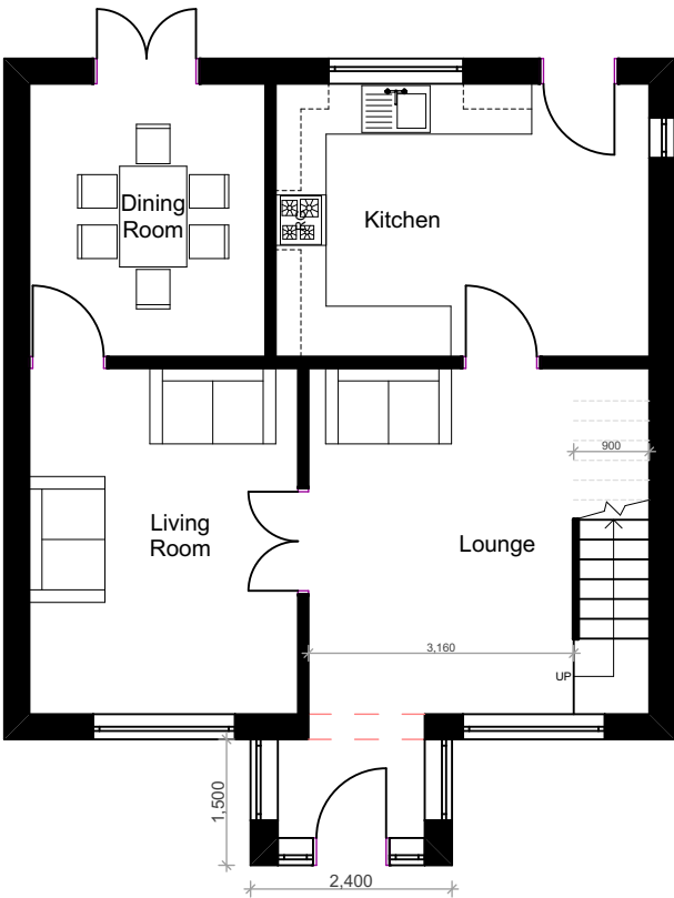
PROPOSED GA GROUND FLOOR PLAN
