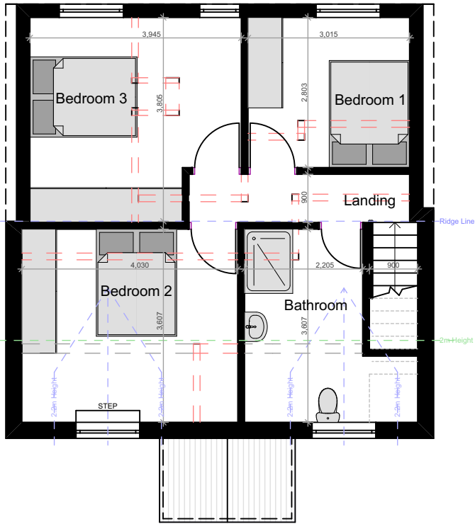
PROPOSED GA FIRST FLOOR PLAN
