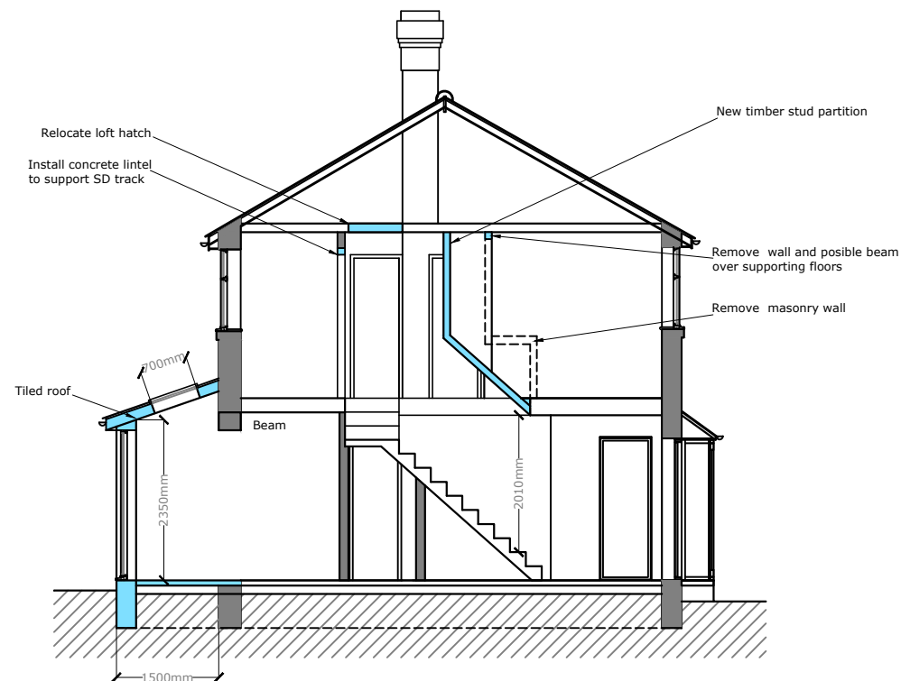
CROSS SECTION
