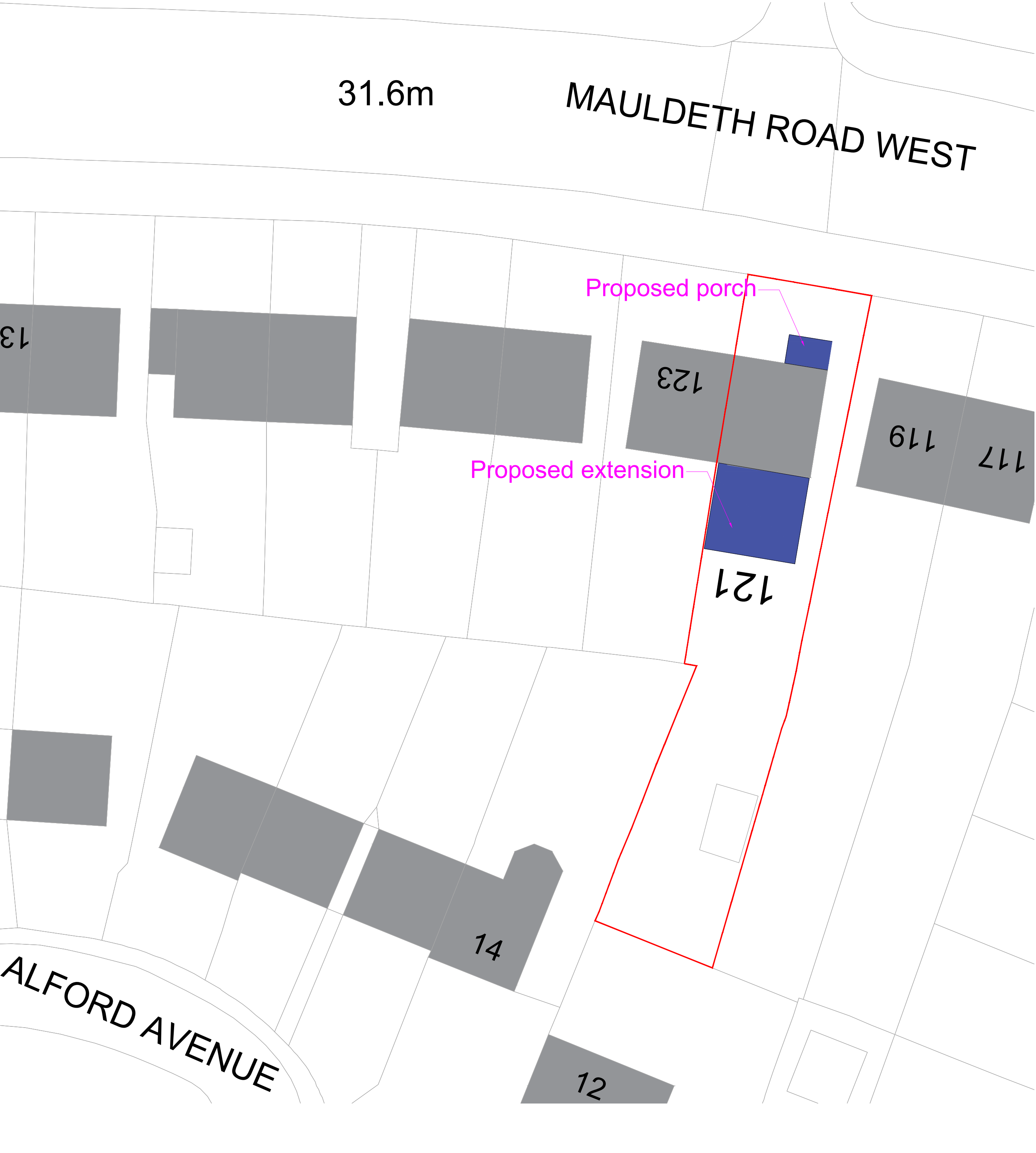
Proposed Site Plan 1:200@A1
