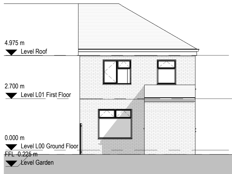
3 Existing East Elevation 1 : 100
