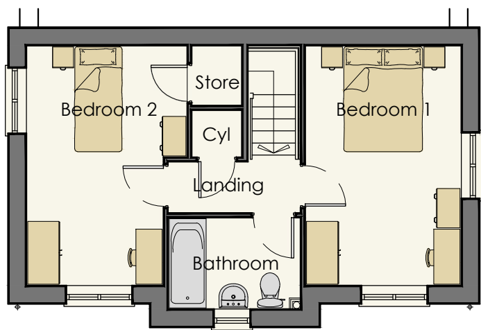
First Floor Plan 2B3P Aspect House Type 77sq.m
