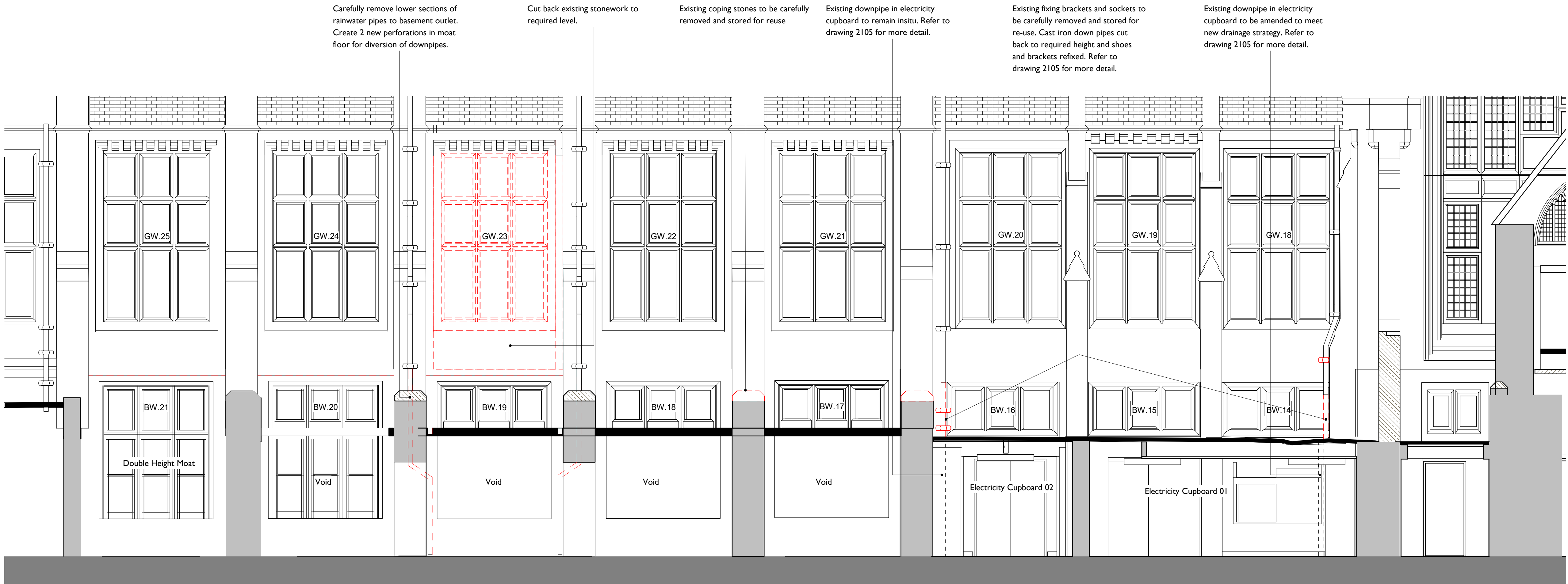
1 Section CC as Existing 1232 1 : 50
