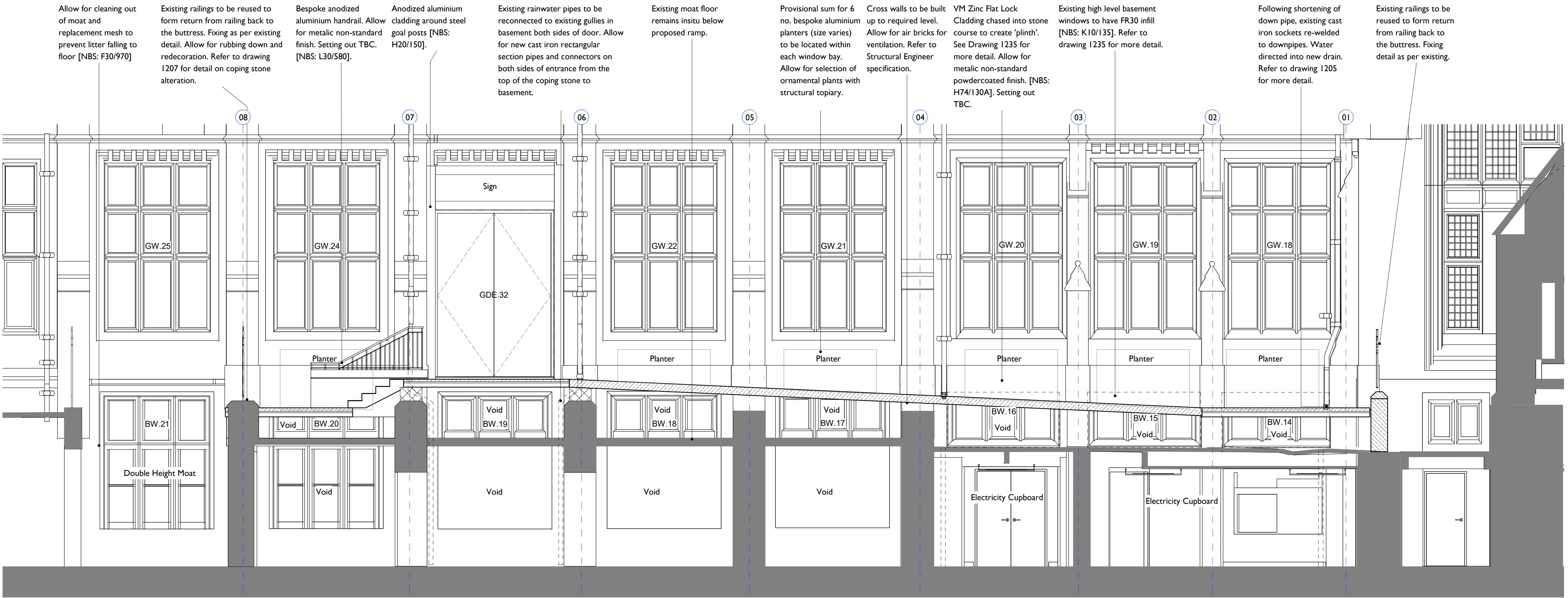
2 Section CC as Proposed 1232 1 : 50
