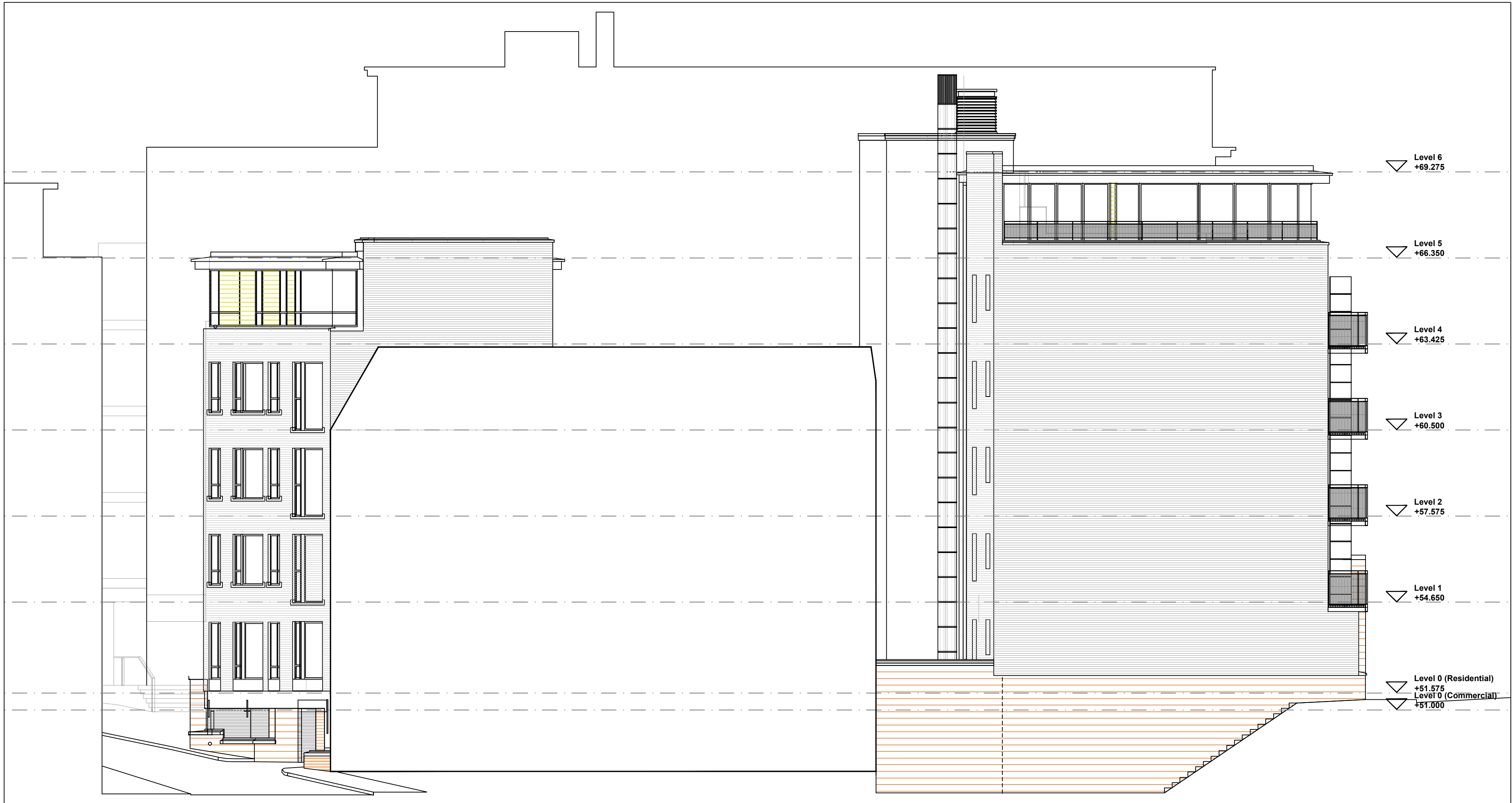
[4] Arena End Elevation 1:100
