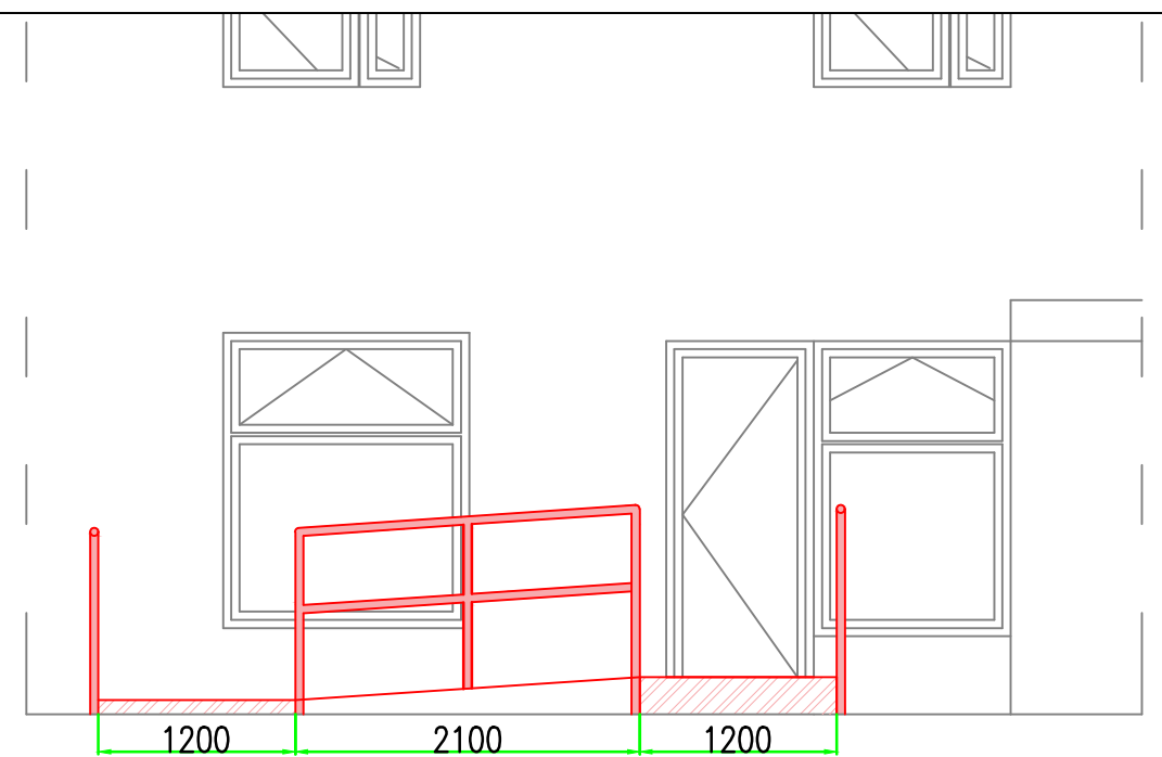
REAR ELEVATION
