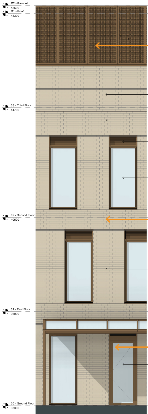
Part Elevation of School. Approved drawing ref C3-AKL-G251-SE-XX-0017 X01
