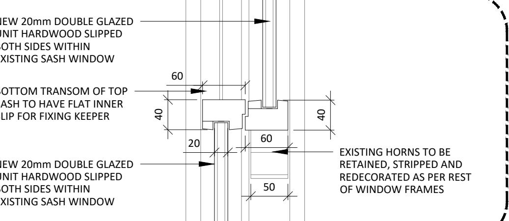
07b TYPE D WINDOW JOINT 513 SCALE 1:5 PROPOSED SECTION
