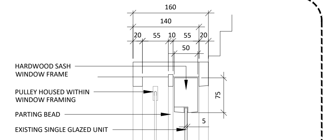
03a TYPE D WINDOW HEAD 513 SCALE 1:5 EXISTING SECTION
