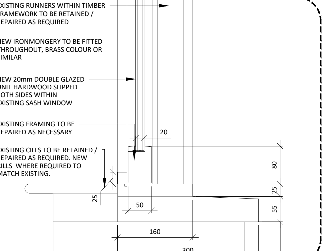
07c TYPE D WINDOW CILL 513 SCALE 1:5 PROPOSED SECTION
