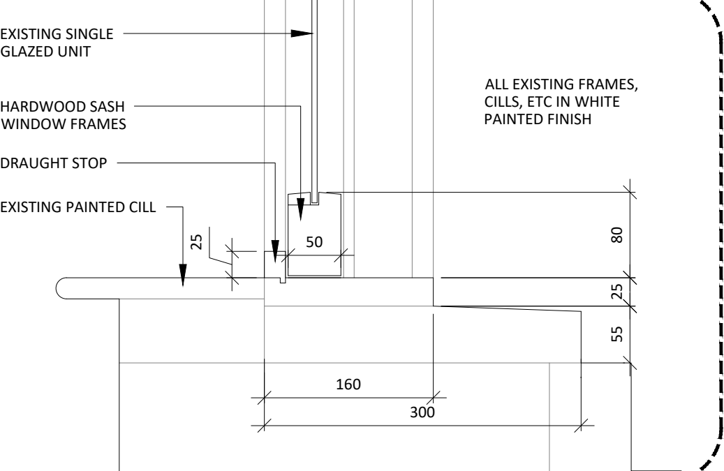
03c TYPE D WINDOW CILL 513 SCALE 1:5 EXISTING SECTION
