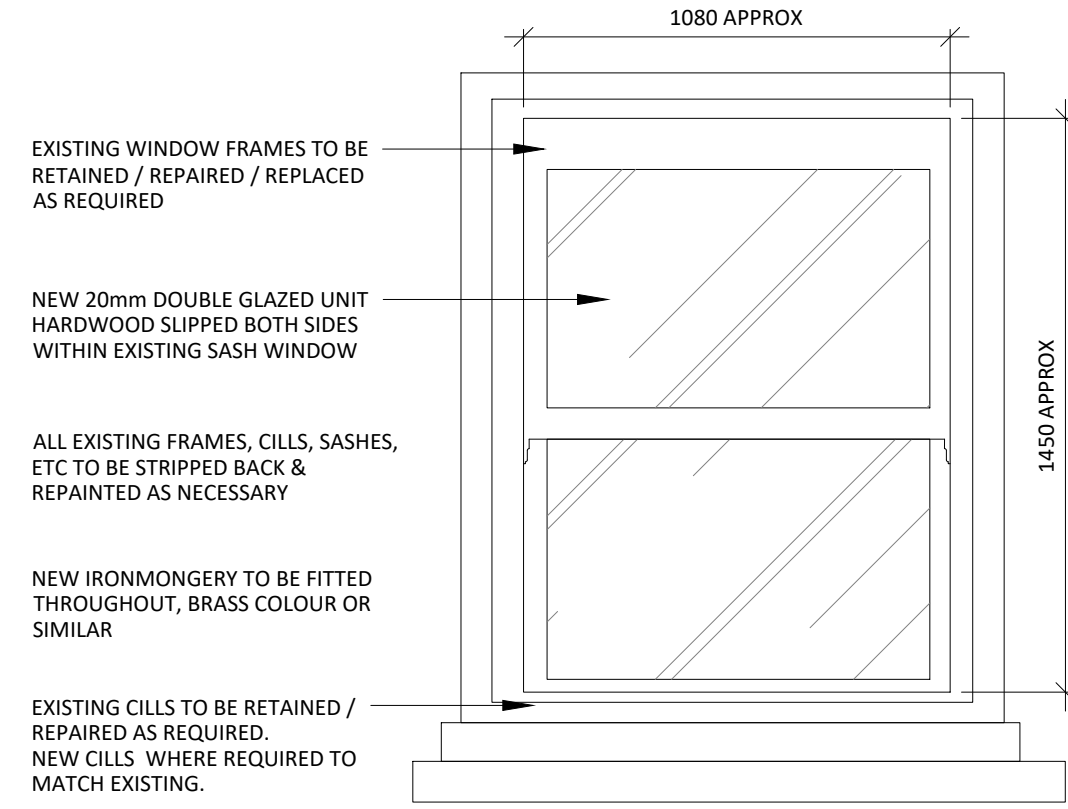
05 4th FLOOR SASH WINDOW - TYPE D 513 SCALE 1:20 PROPOSED ELEVATION
