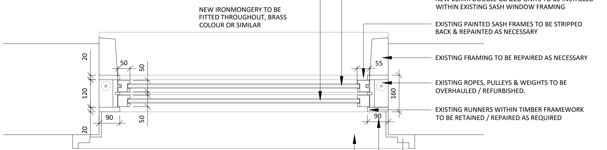
08 1st FLOOR SASH WINDOW - TYPE D 513 SCALE 1:10 PROPOSED PLAN SECTION
