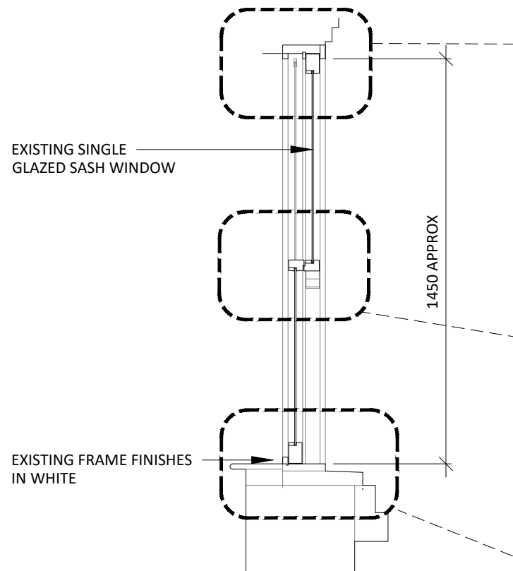
02 4th FLOOR SASH WINDOW - TYPE D 513 SCALE 1:20 EXISTING SECTION
