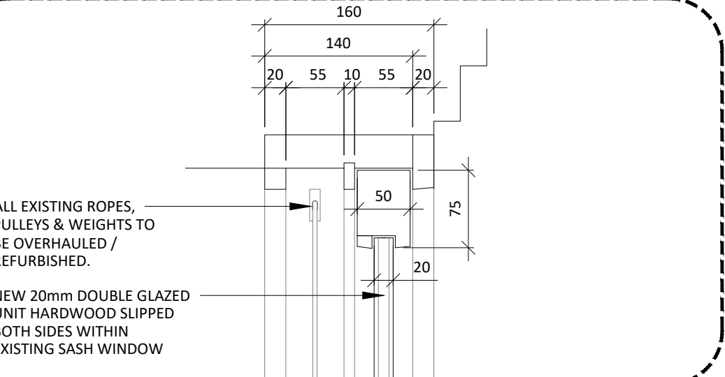
07a TYPE D WINDOW HEAD 513 SCALE 1:5 PROPOSED SECTION
