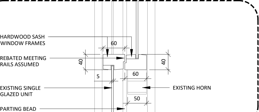
03b TYPE D WINDOW JOINT 513 SCALE 1:5 EXISTING SECTION
