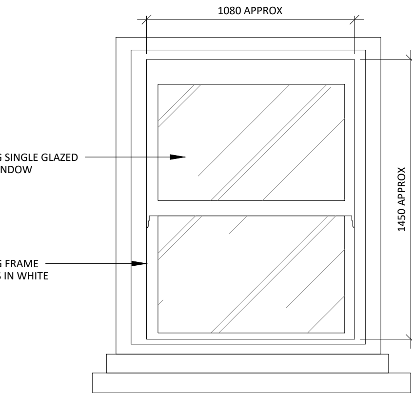
01 4th FLOOR SASH WINDOW - TYPE D 513 SCALE 1:20 EXISTING ELEVATION
