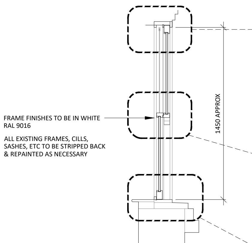
06 4th FLOOR SASH WINDOW - TYPE D 513 SCALE 1:20 PROPOSED SECTION
