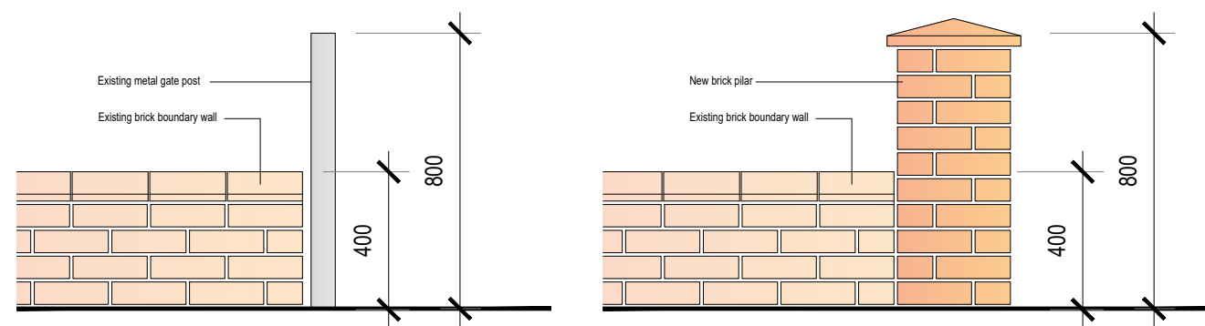
• Detail 1 Existing boundary wall and post detail
