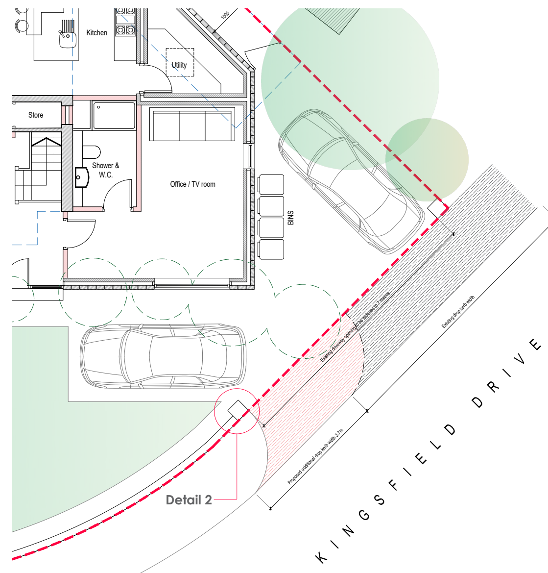
• Proposed driveway entrance plan
