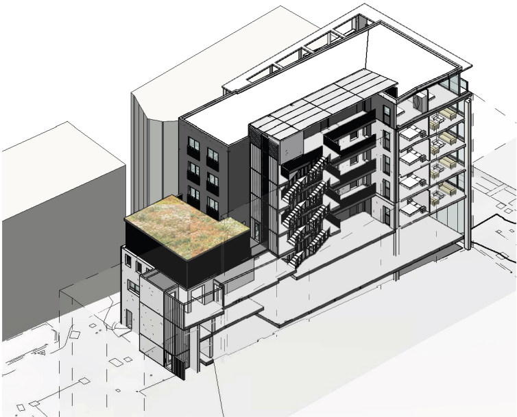
Rear Elevation Perspective 1
