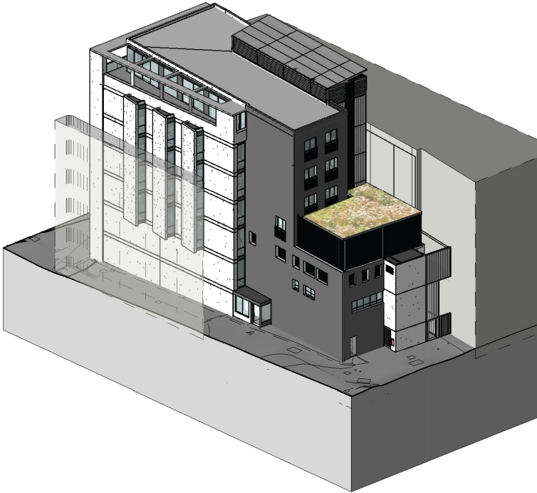
Rear Elevation Perspective 2
