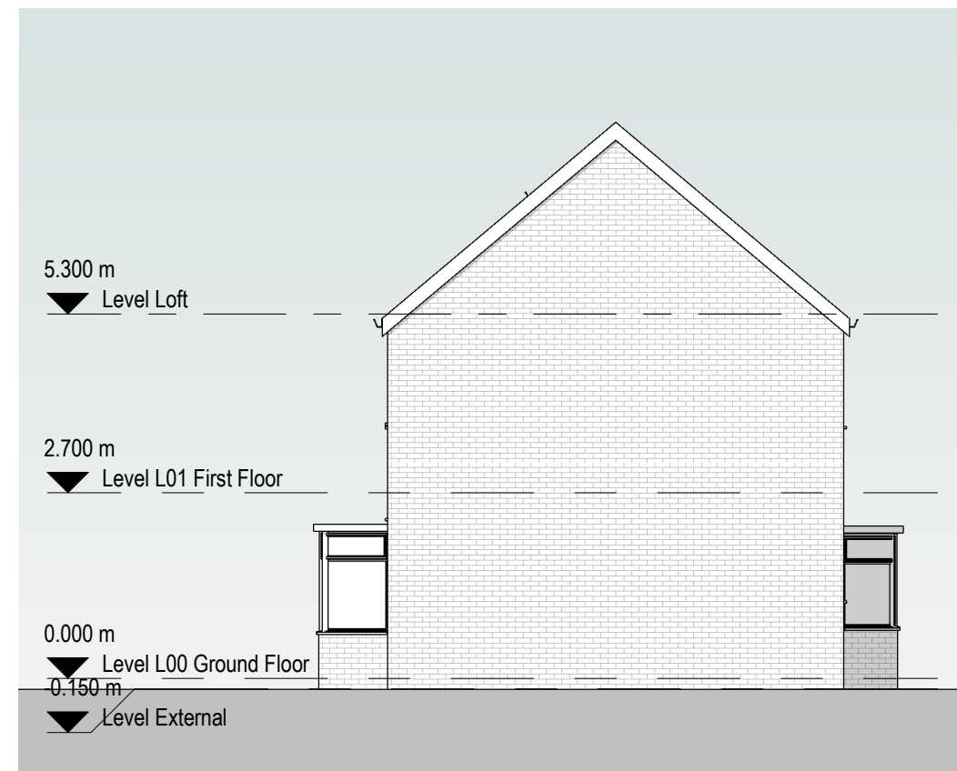
4 Existing East Elevation 1 : 100
