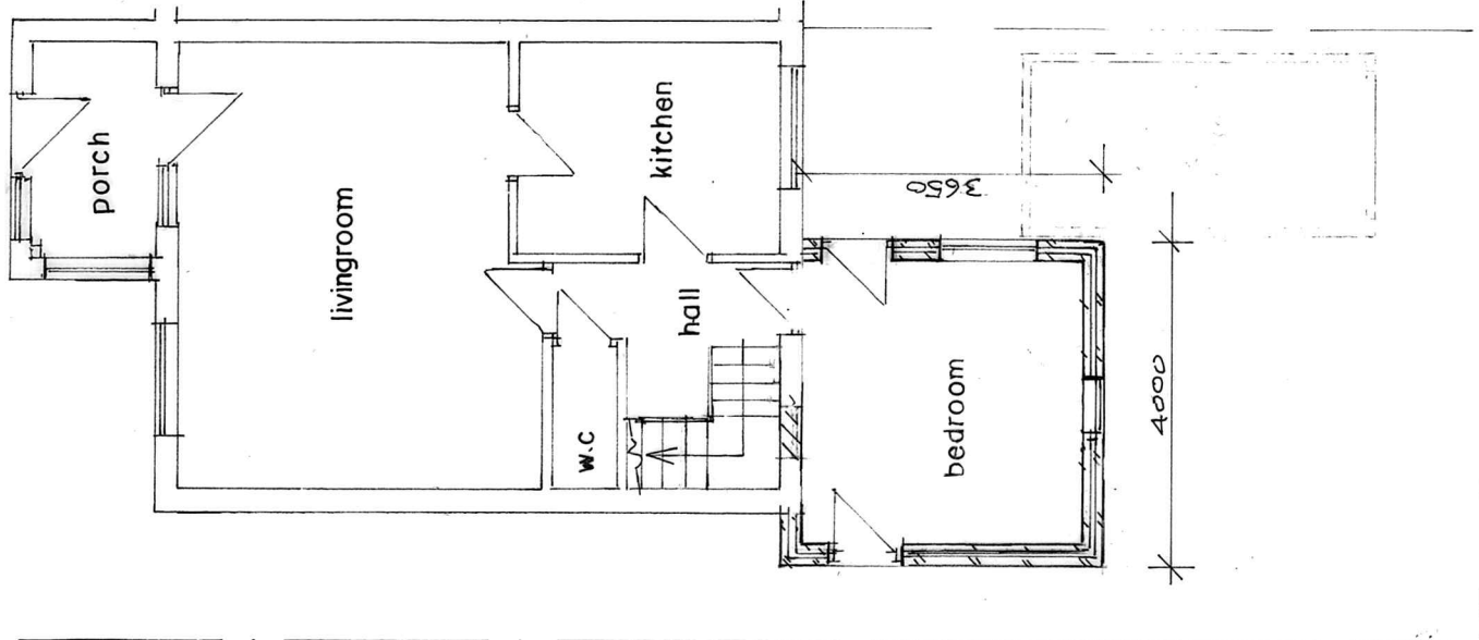
GROUND FLOOR PLAN (PROPOSED)
