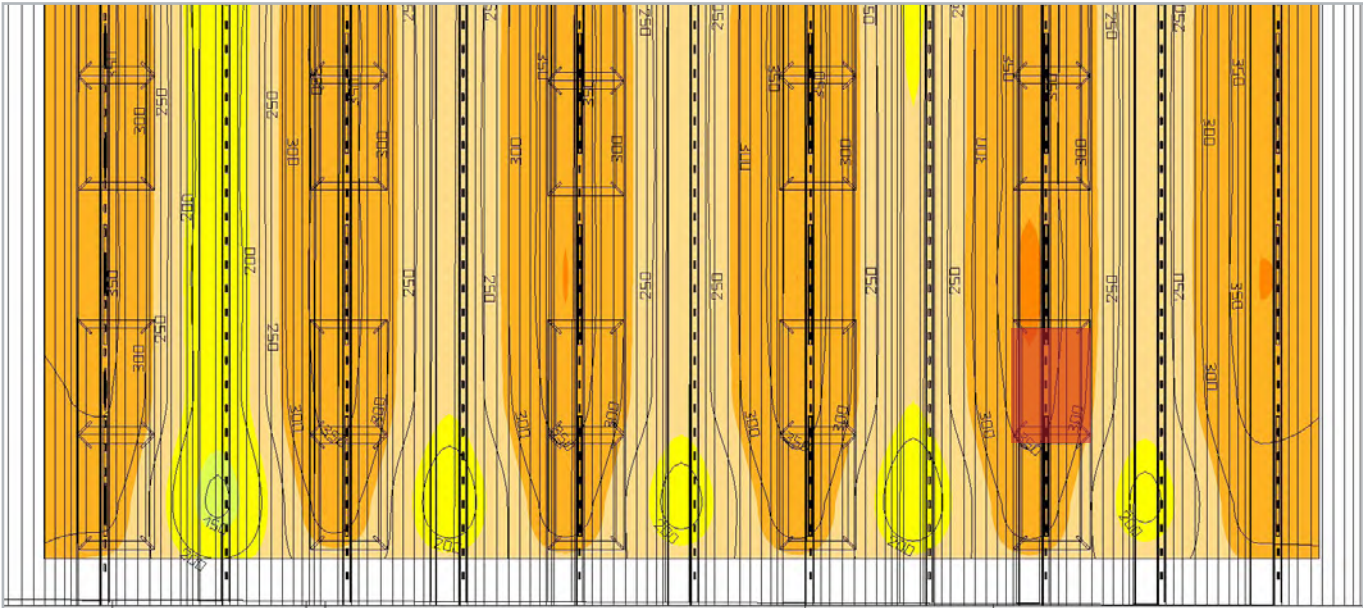
Custom profile with Fagerhult, Eavg=291lm; Good Uniformity 0.49, Desk Uniformity 0.98, Approx 5.5W/m²
