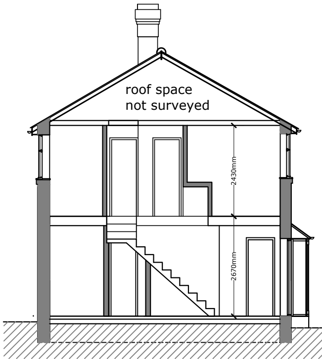
CROSS SECTION
