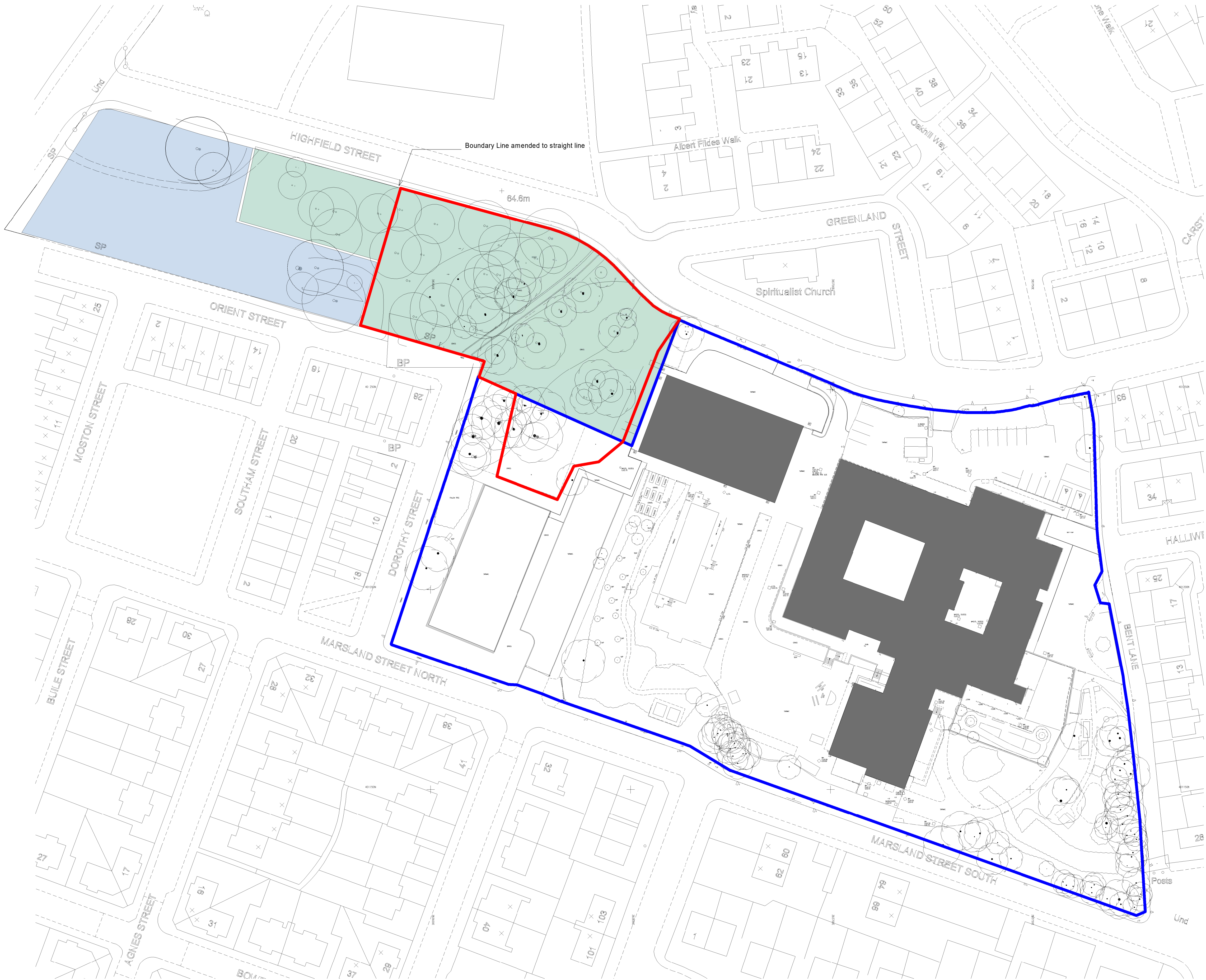
Block Plan, showing area of works and current land ownership scale 1:500 @A1
