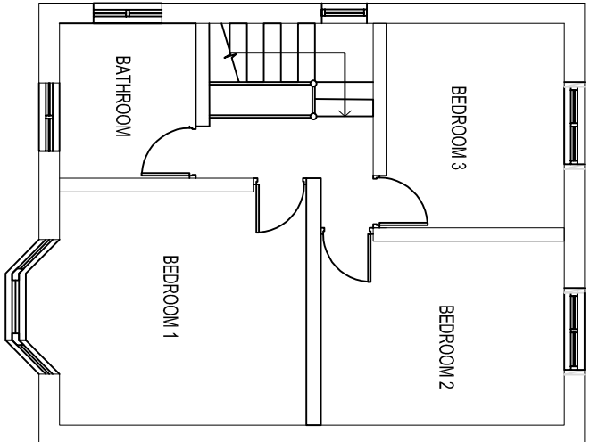
EXISTING FIRST FLOOR PLANE 1:100
