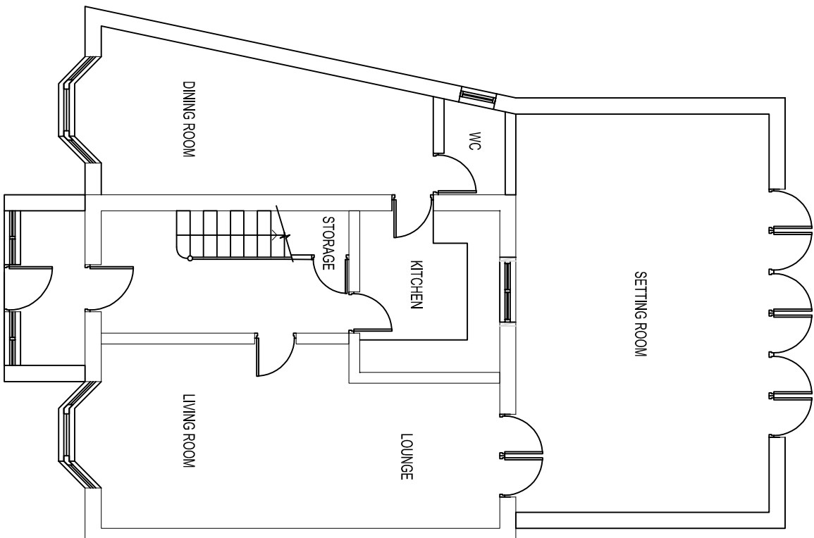
PROPOSED GROUND FLOOR PLANE 1:100
