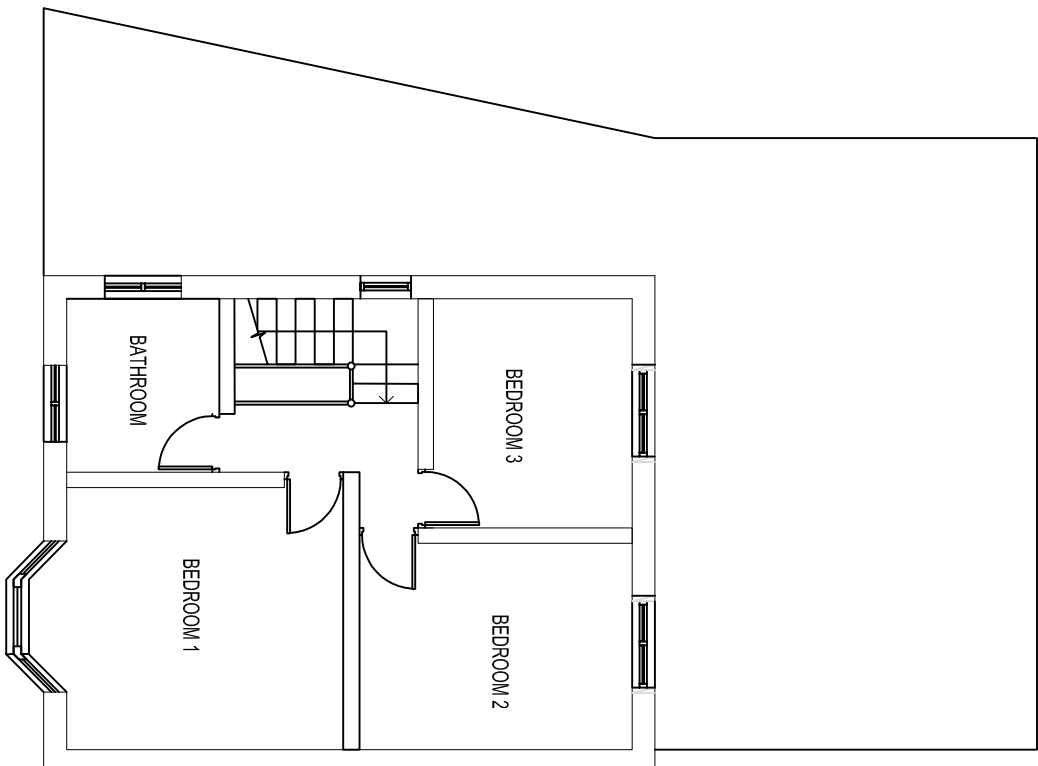
PROPOSED FIRST FLOOR PLANE 1:100
