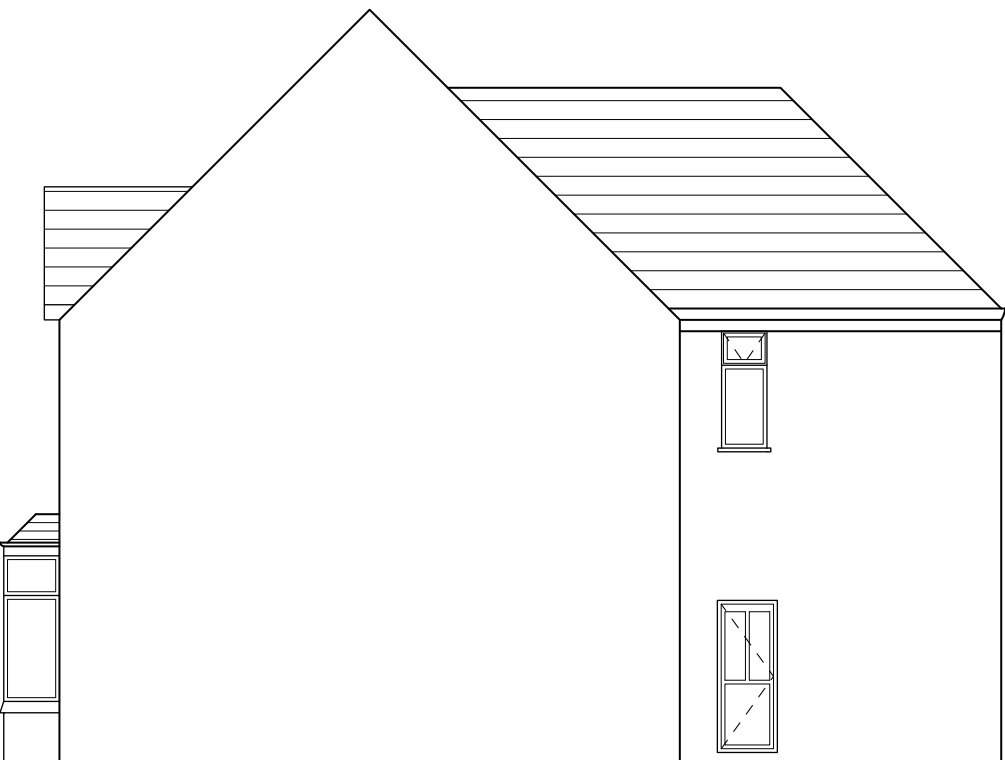
SOUTH ELEVATION SCALE 1:100 UID - P007
