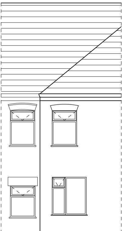
EAST ELEVATION SCALE 1:100 UID - P006
