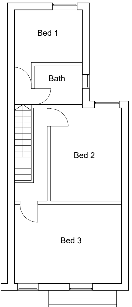
FIRST FLOOR SCALE 1:100 UID - P004
