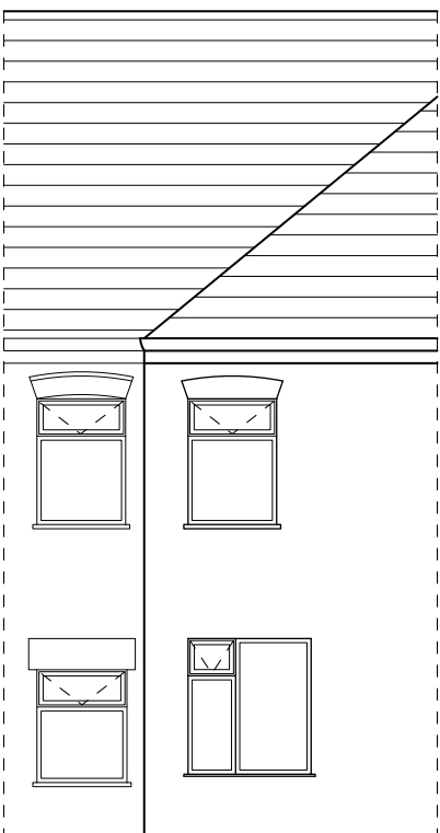
EAST ELEVATION SCALE 1:100 UID - E006
