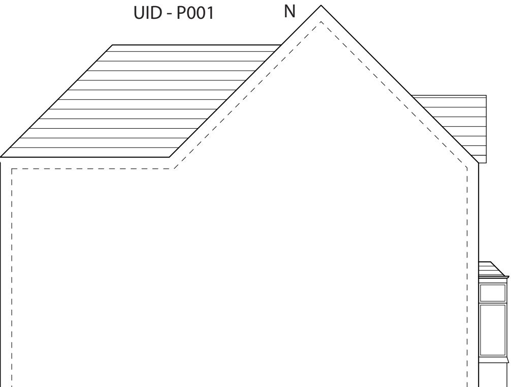
NORTH ELEVATION SCALE 1:100 UID - E008
