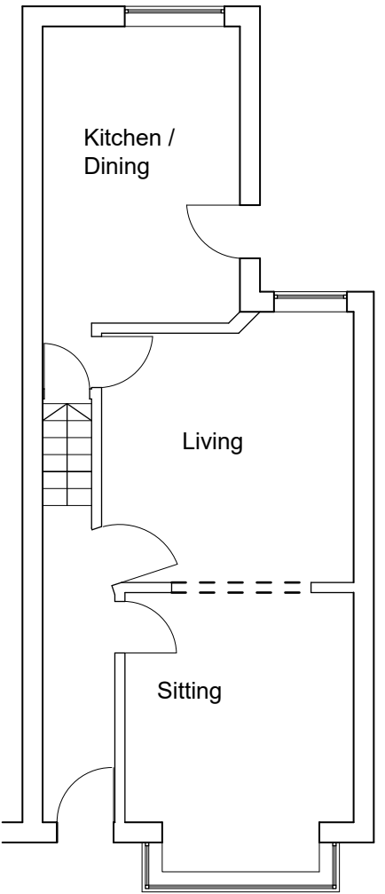
GROUND FLOOR SCALE 1:100 UID - E003
