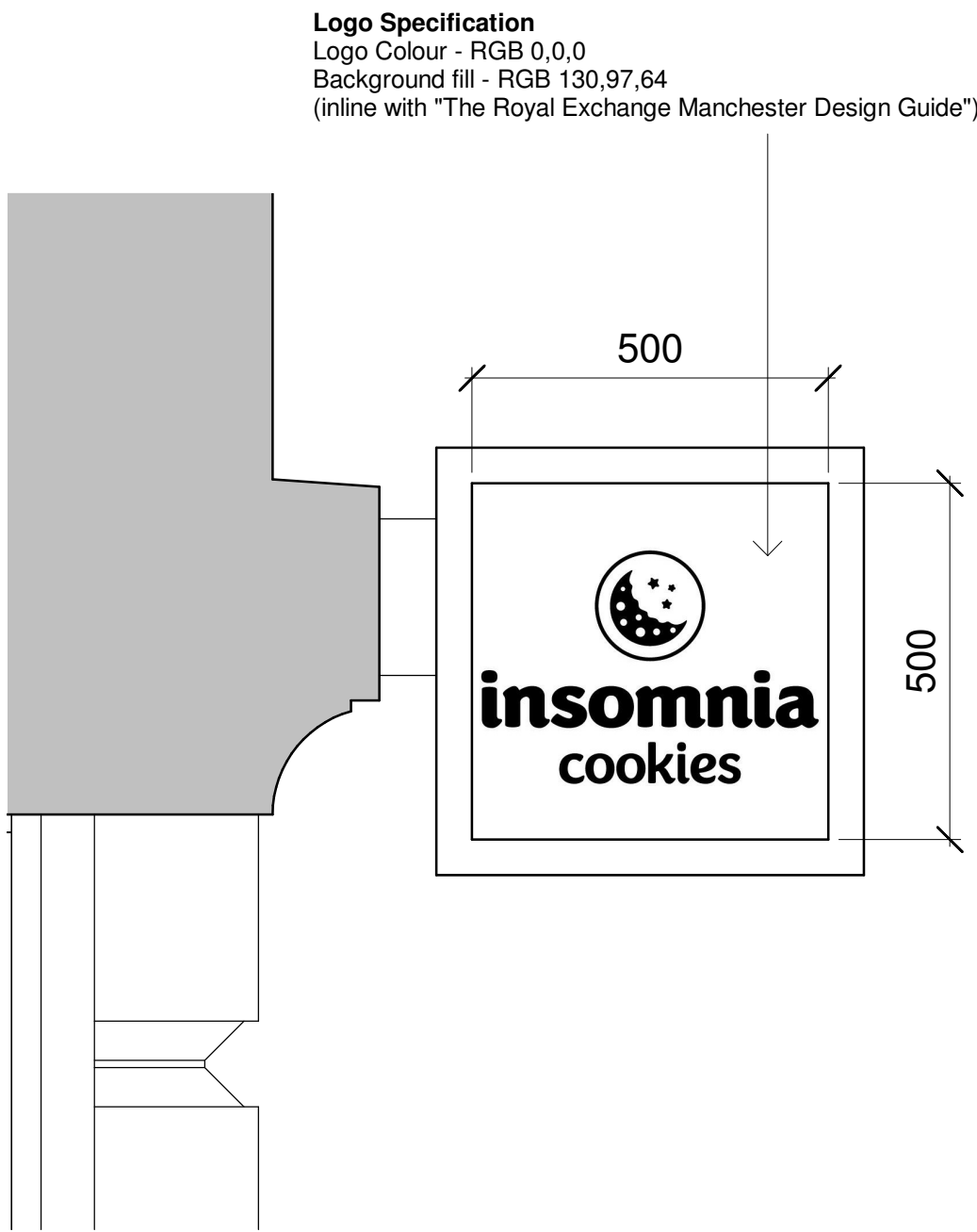
Proposed back illuminated signage 1 : 10
