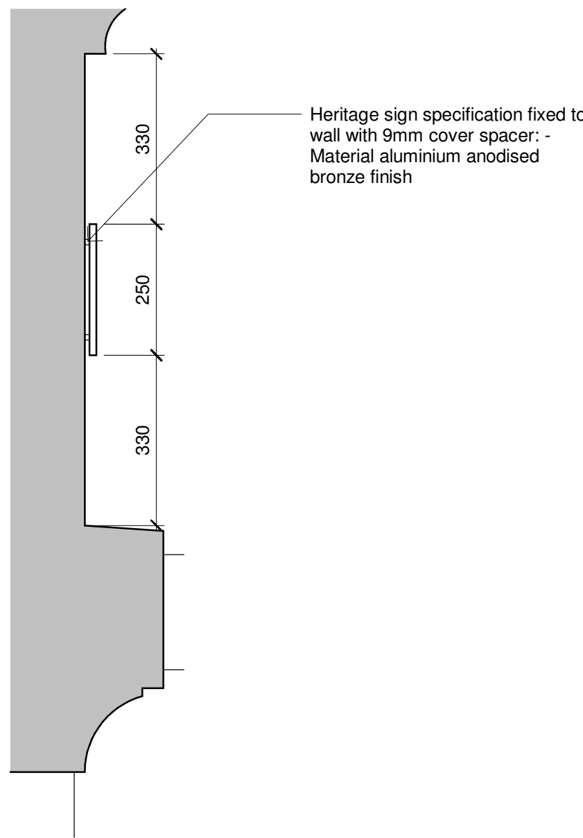
Proposed fixed sign - Section 1 : 10
