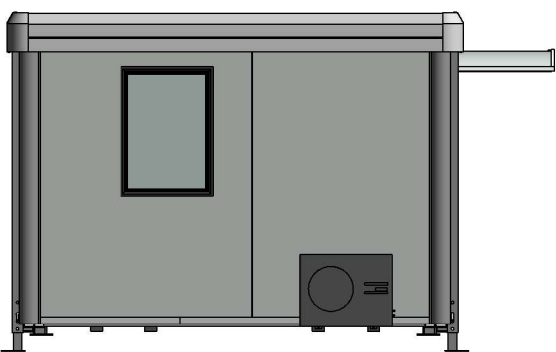
Side Elevation 1 : 70
