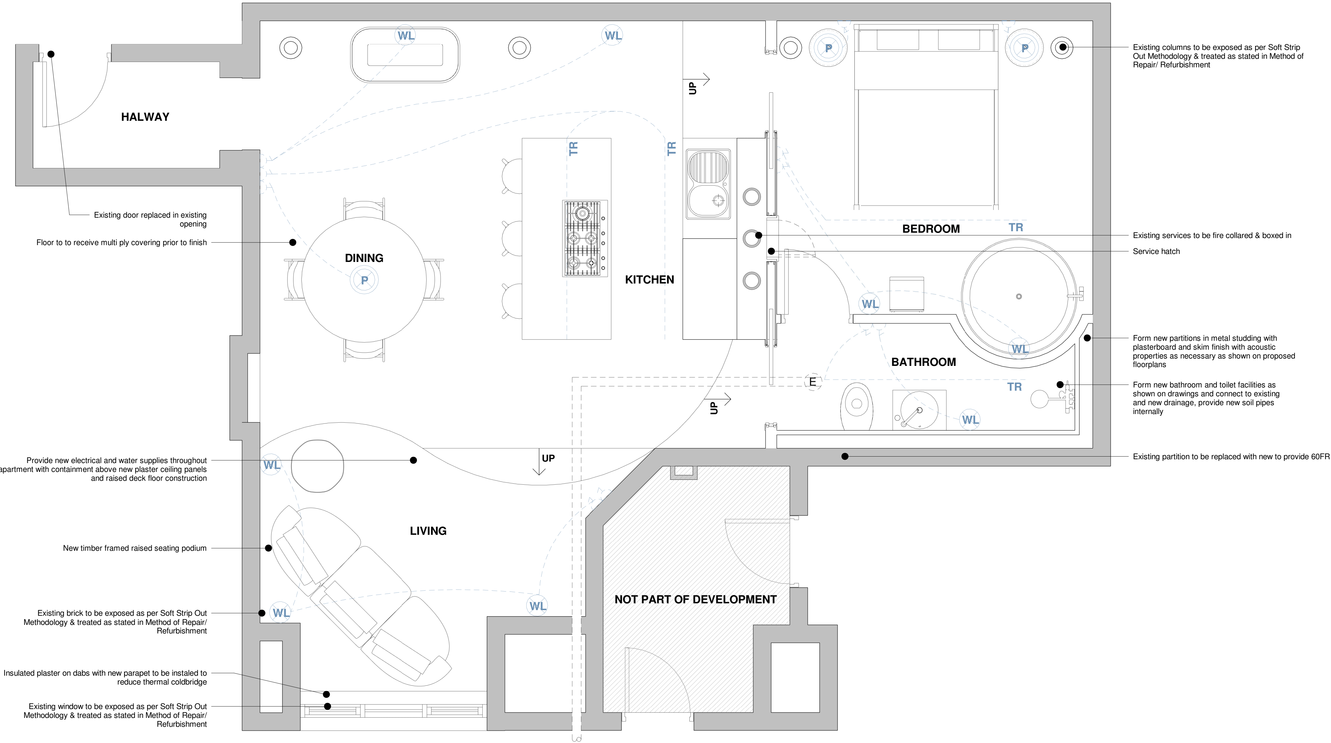
00 - Proposed Ground Floor Level Scale: 1 : 25
