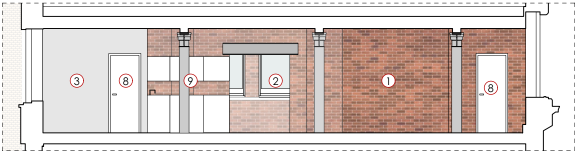
FOURWAYS HOUSE, FOURTH FLOOR EXISTING SECTION HH'
