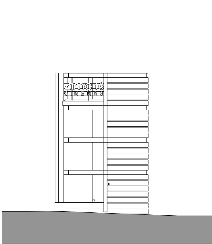
02 North Elevation: Phase 01 Gable End
