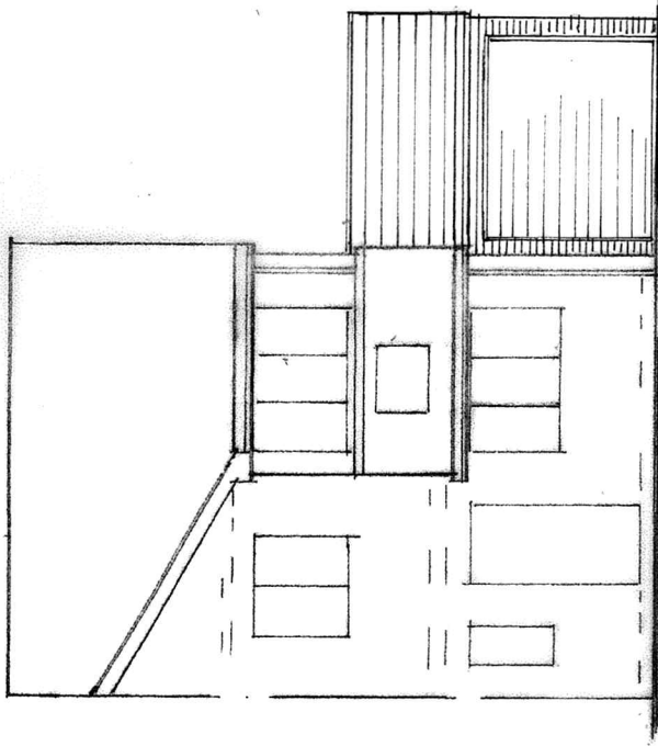
FRONT ELEVATION (PROPOSED)
