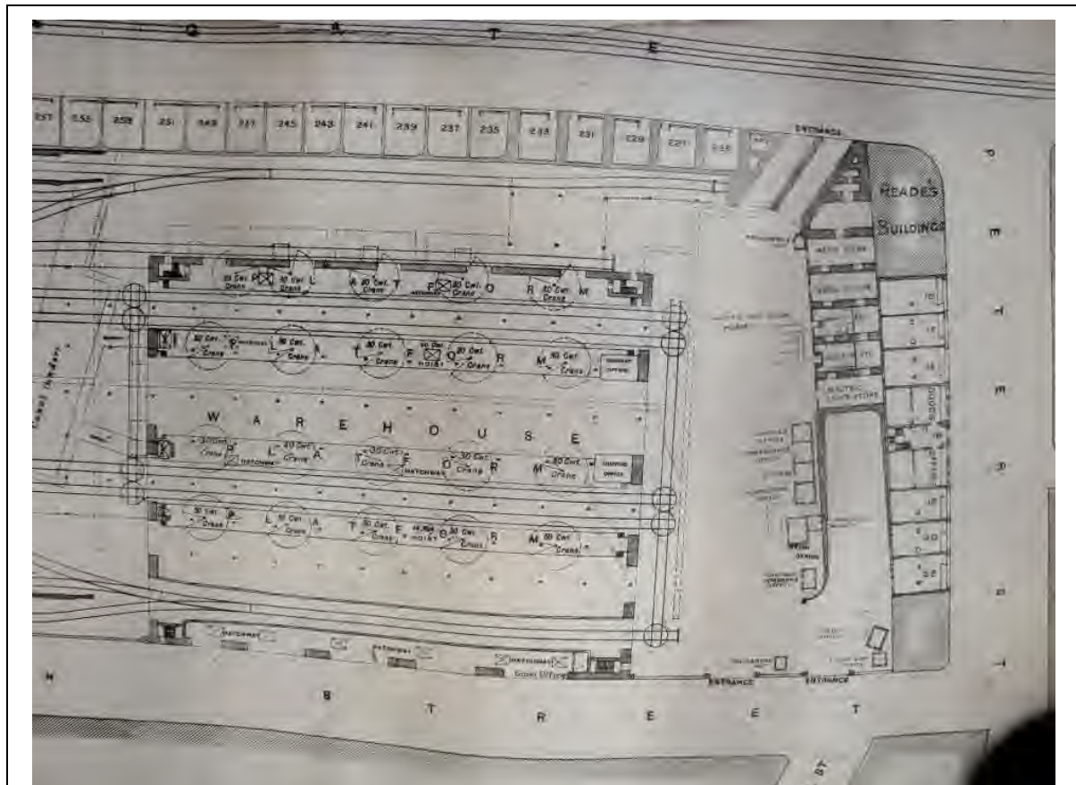
Figure 32 – Plan of the low level station (ground floor), showing Peter Street to the right, 1897.
