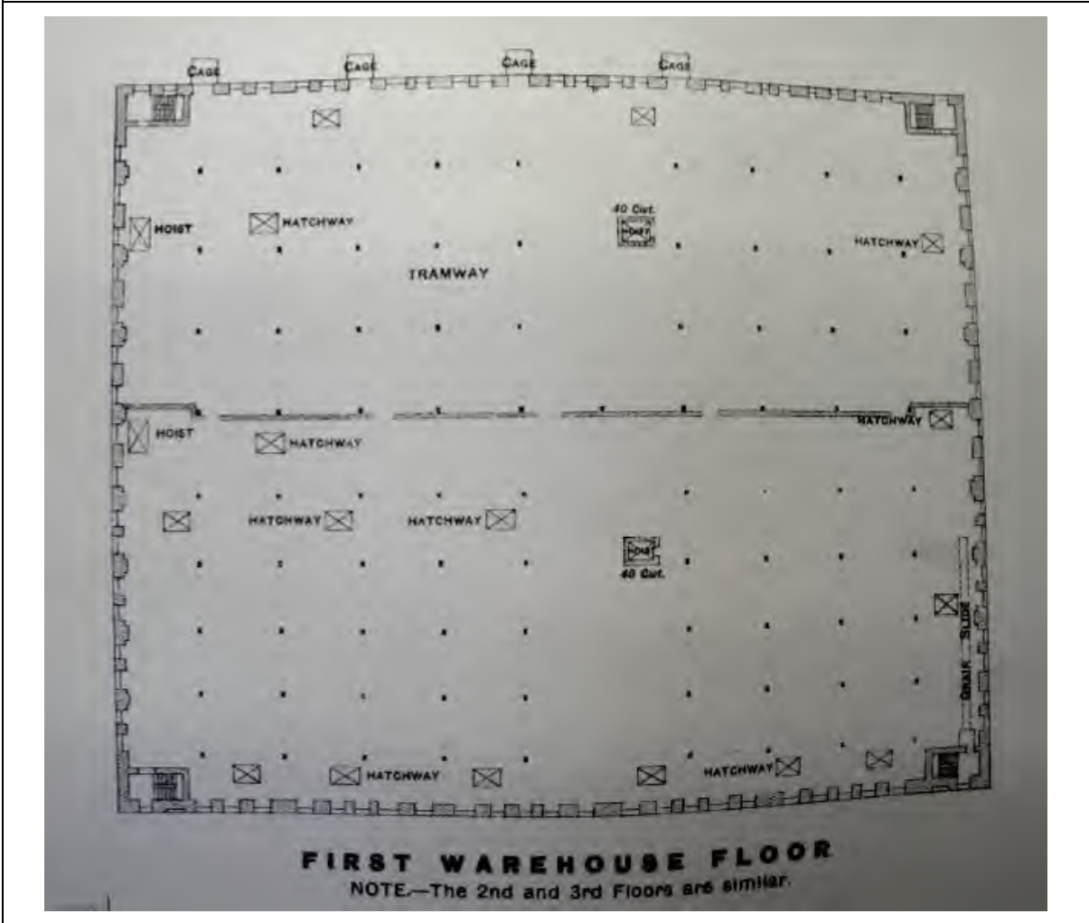
Figure 35 – First warehouse floor plan, 1897, (second floor on the present building arrangement)
