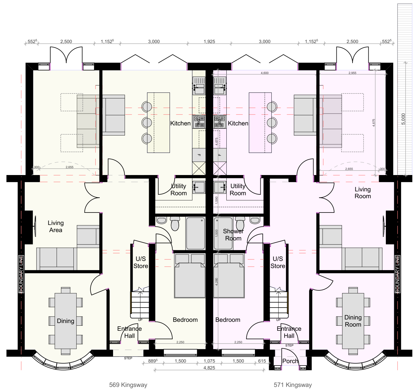
PROPOSED GA GROUND FLOOR PLANS
