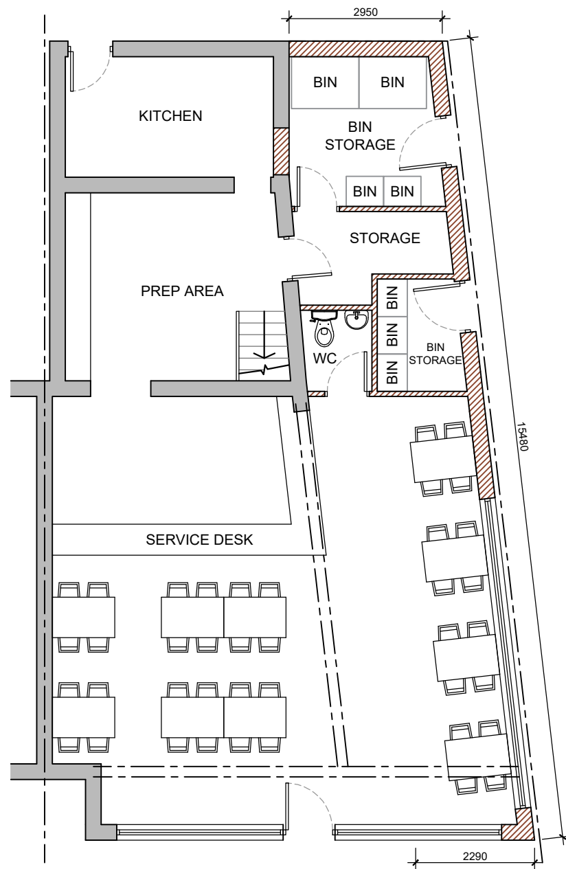
GROUND FLOOR 1:100
