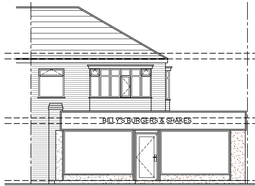
FRONT ELEVATION 1:100
