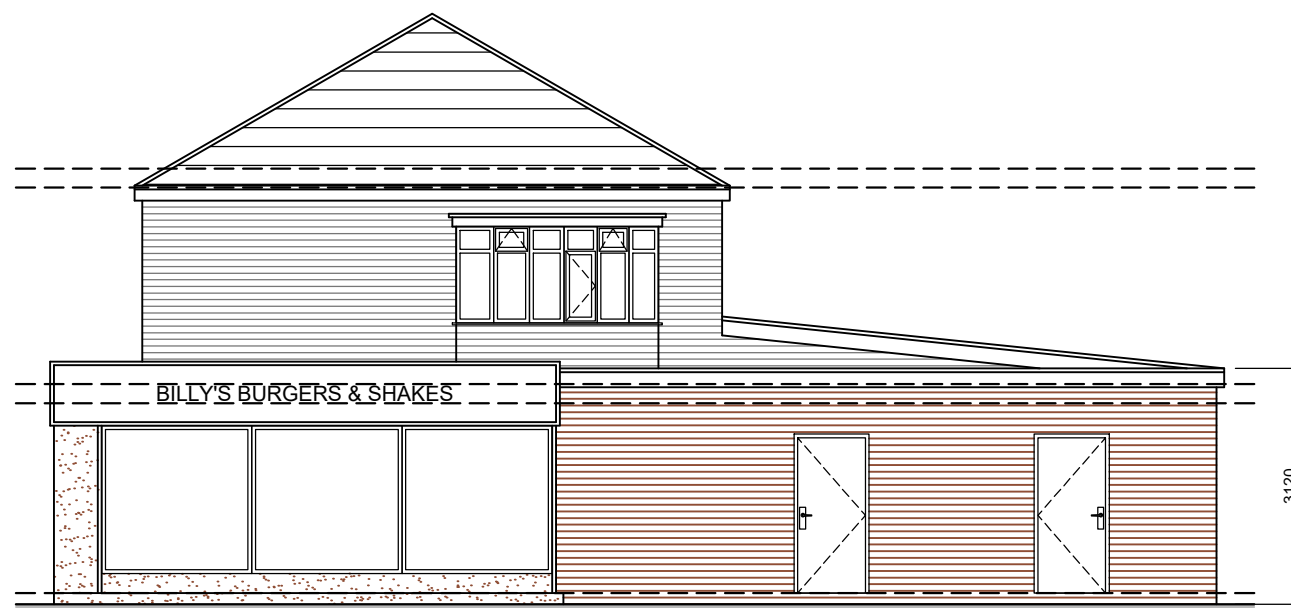
SIDE ELEVATION 1:100
