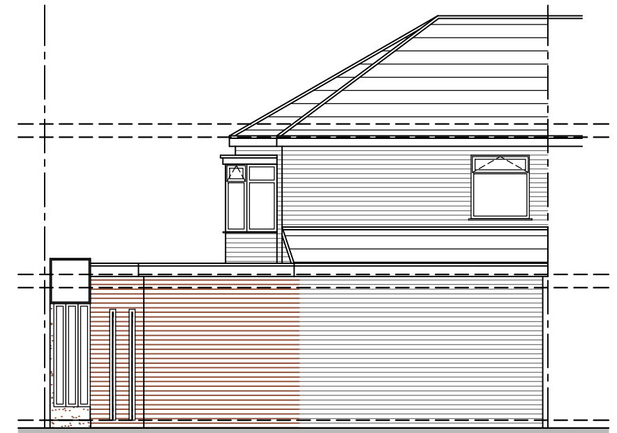
REAR ELEVATION 1:100
