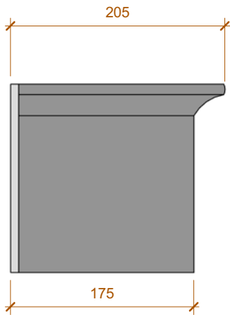
Side Elevation 1:5
