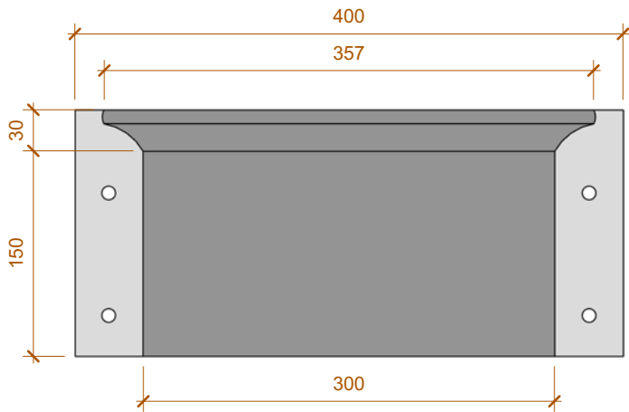
Front Elevation 1:5
