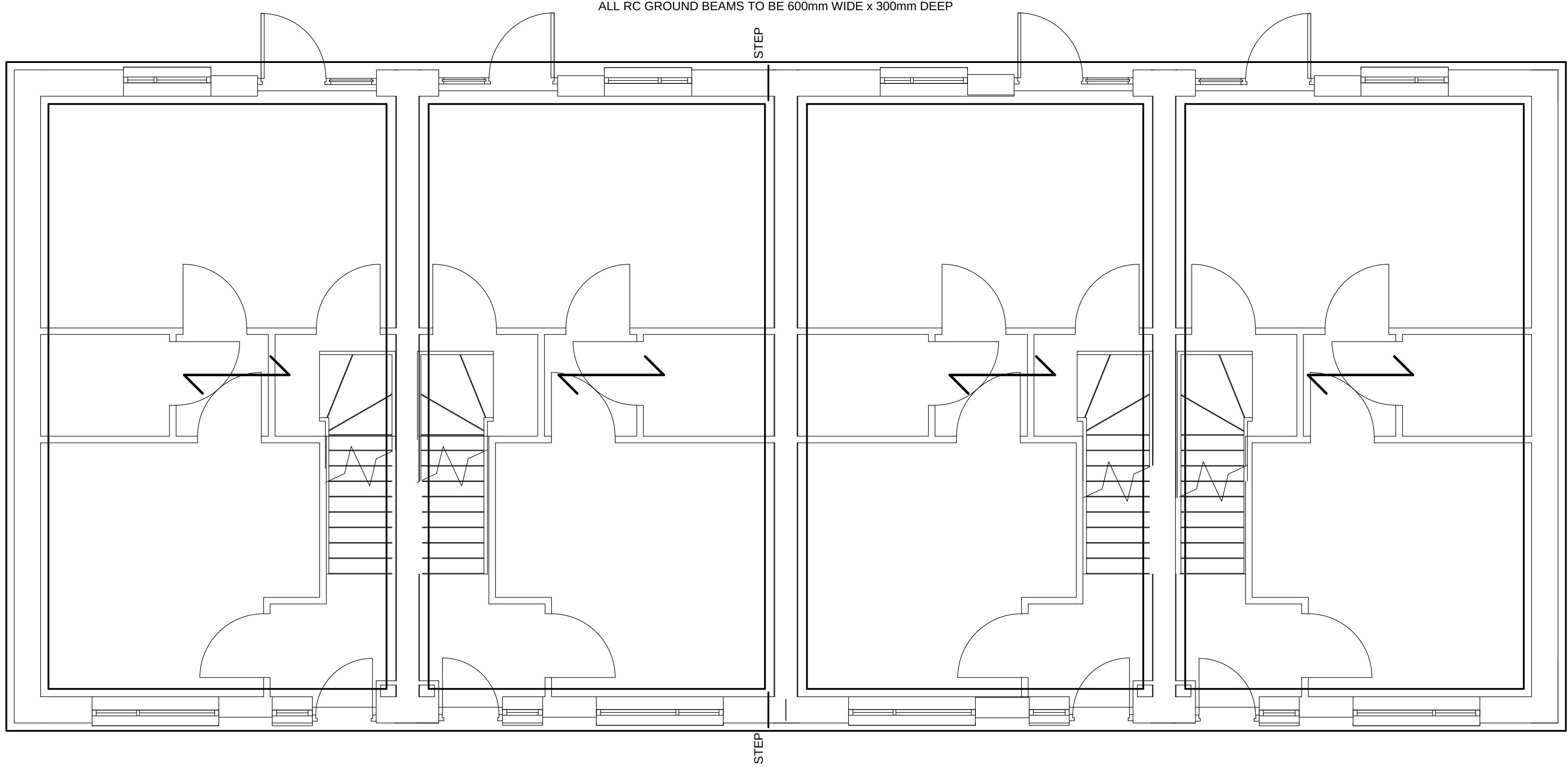
BLOCK 1
