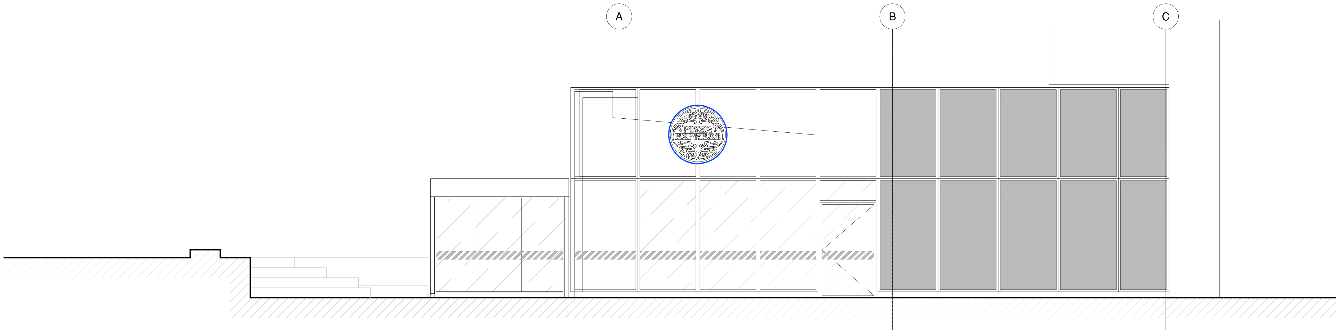
01 EXISTING SIDE (WEST) ELEVATION 51 SCALE 1:50
